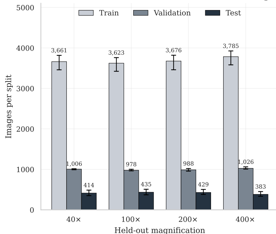
(b) Images per split, mean over 3 seeds (whiskers = min-max; train/val from the 3 training mags)
