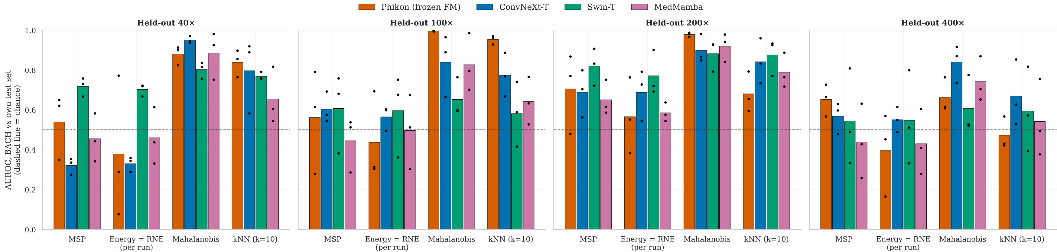
Separating another institution (BACH) from the held-out BreakHis test set, per held-out magnification (bars = mean, dots = seeds)
