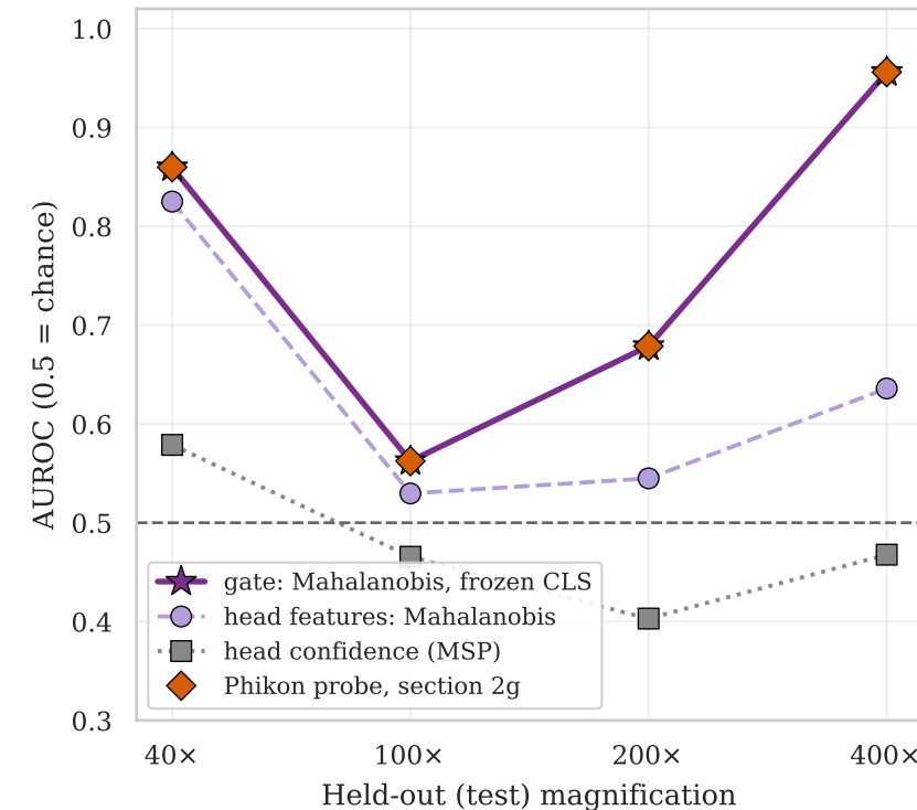
(c) Detecting the shift: unseen magnification vs validation
