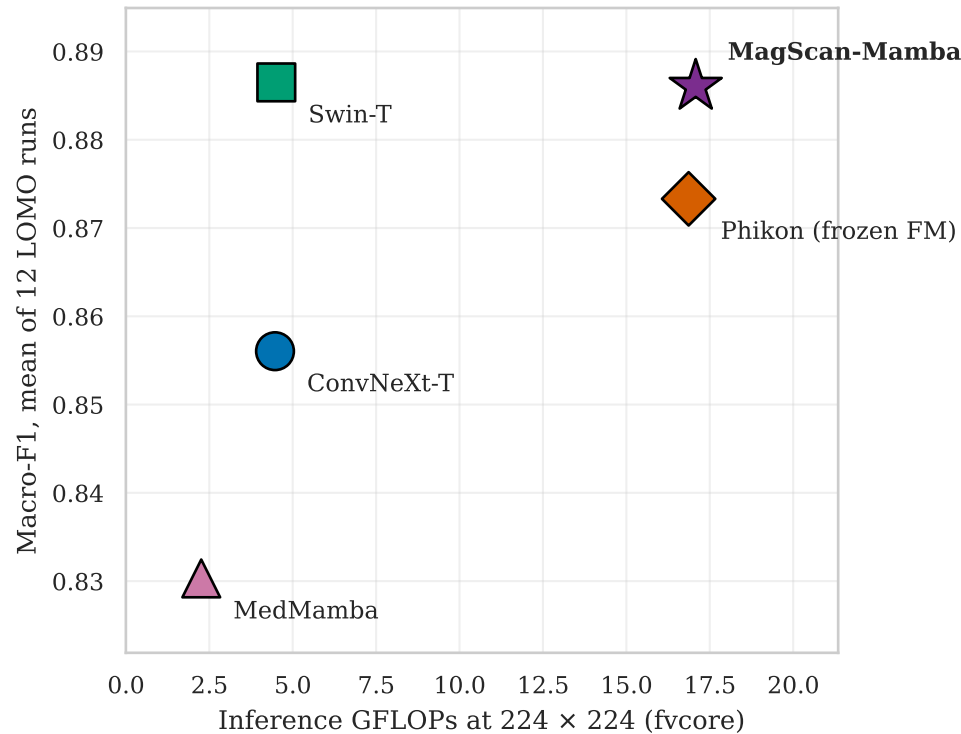
(a) Macro-F1 (higher is better) against compute
