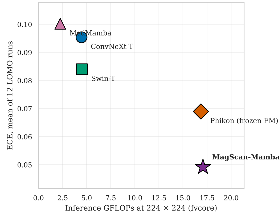
(b) ECE (lower is better) against compute
