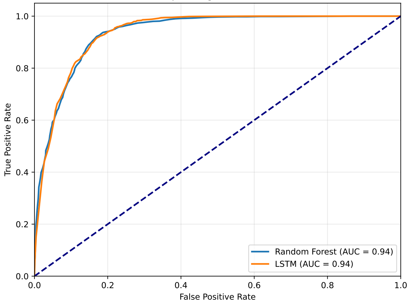
Receiver Operating Characteristic (ROC)
