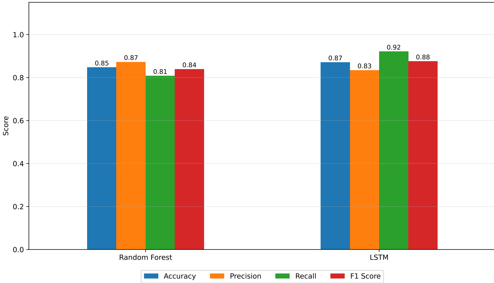
Model Performance Metrics Comparison
