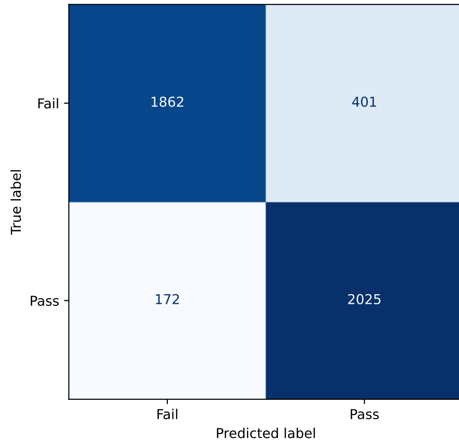
LSTM Confusion Matrix
