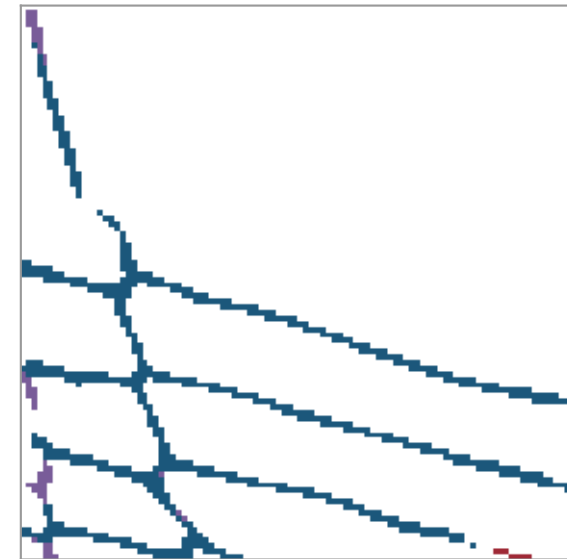
\tau = 3 F1@3 0.955
