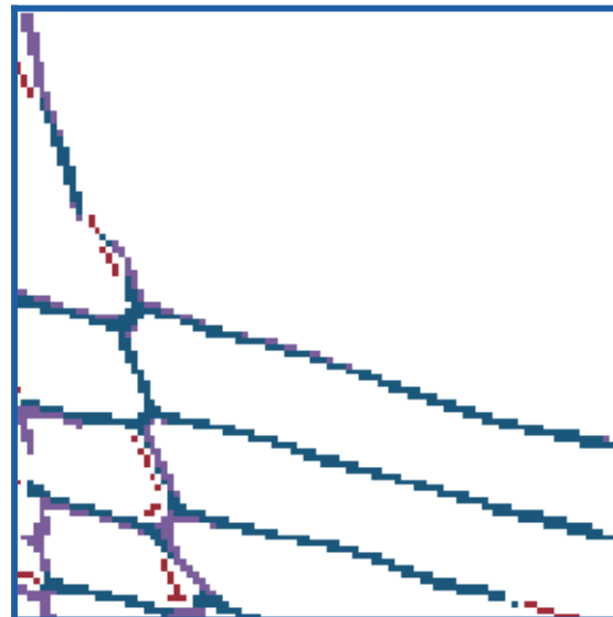
\tau = 1 F1@1 0.792
