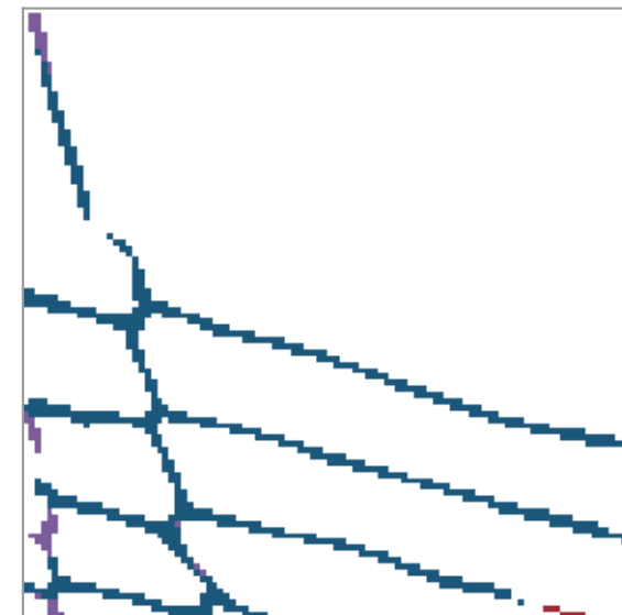
\tau = 3 F1@3 0.955
