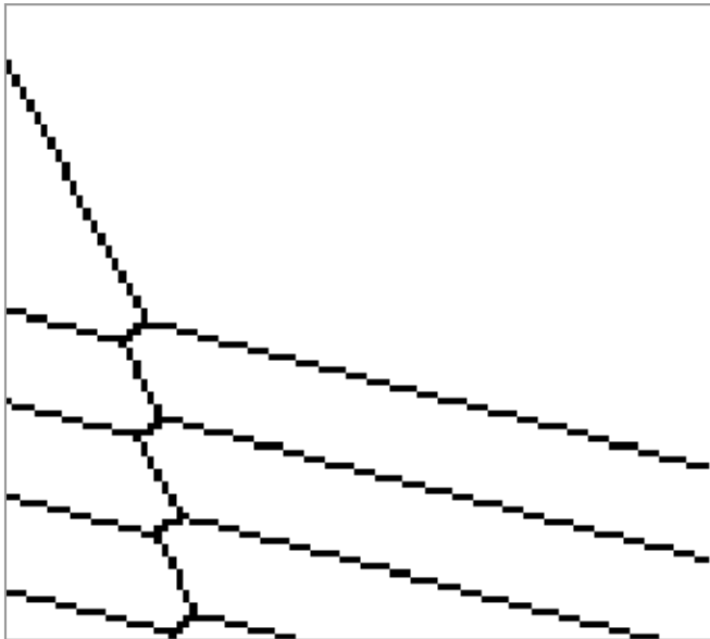
stability diagram (ground truth)
