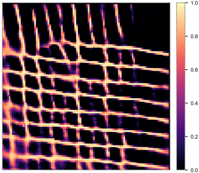
U-Net output P(transition line)
