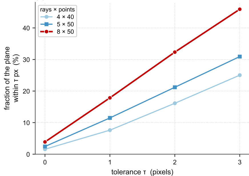
(a) what \tau costs
