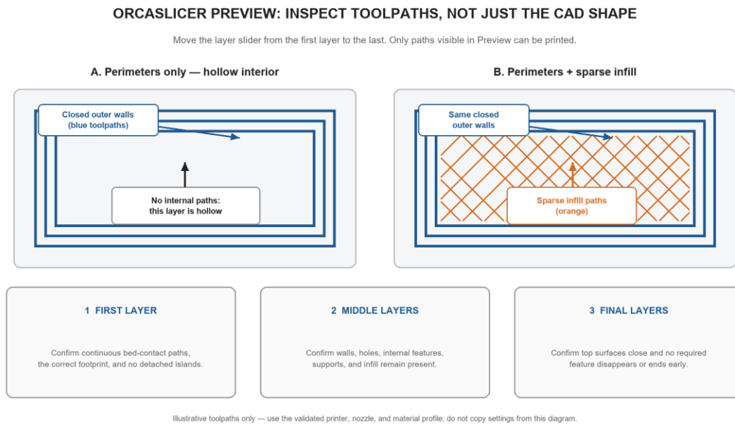
Figure 1. How to read Preview. Blue paths are closed perimeters; orange paths are sparse infill. Infill changes the interior but cannot repair a missing perimeter. Inspect first, middle, and final layers, and use only a validated printer, nozzle, material, and process profile.
