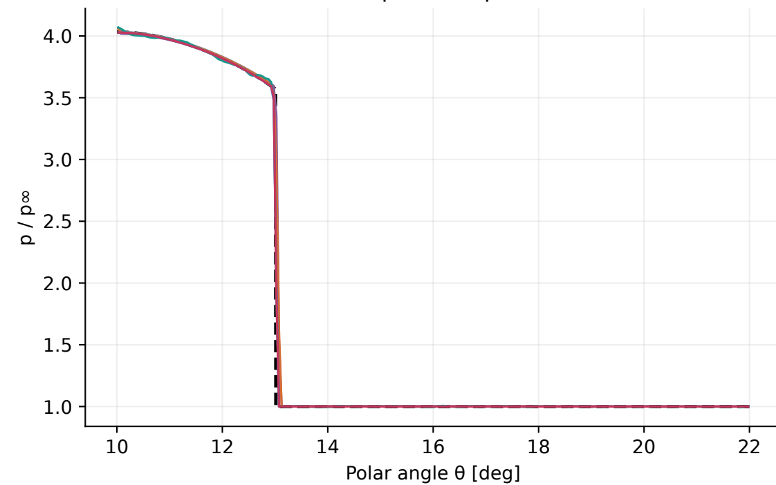
M_\infty=7.95 : full pressure profile, N=240
