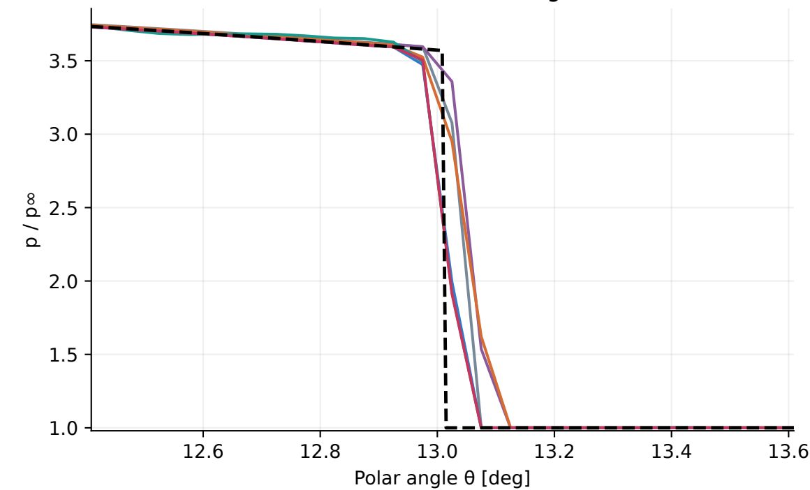
M_\infty=7.95 : resolved shock neighborhood
