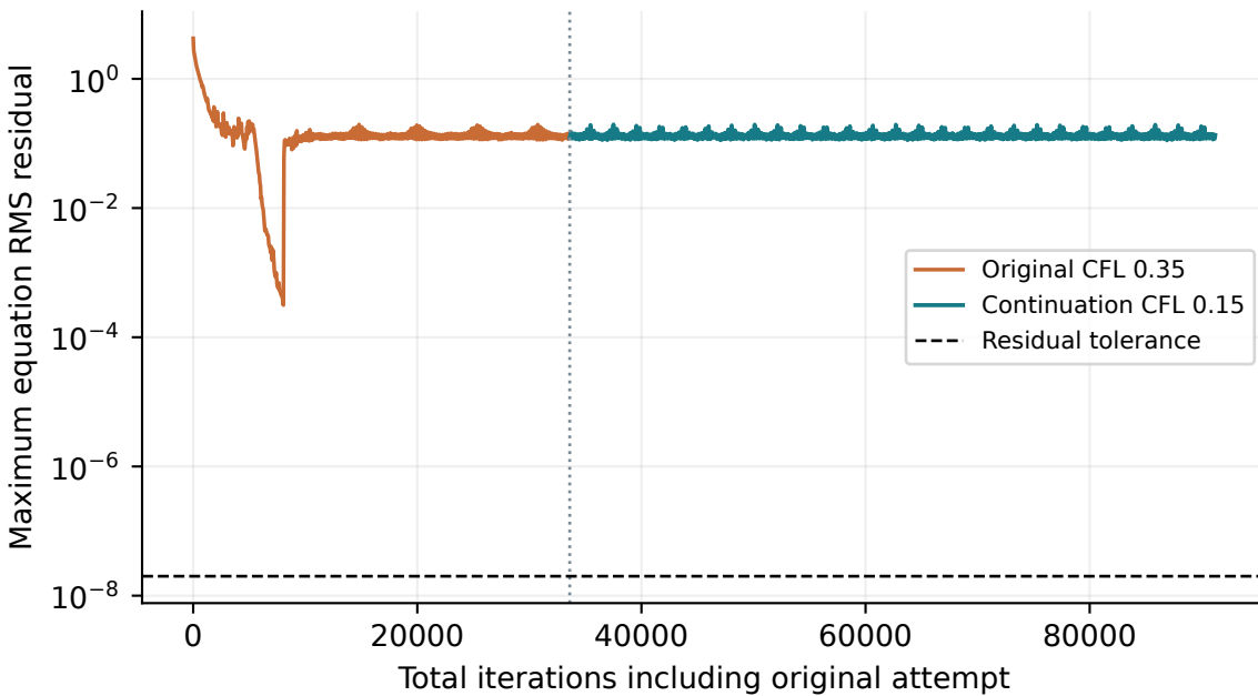
M_\infty=7.95 , N=60 : HLLC / MUSCL-MC
