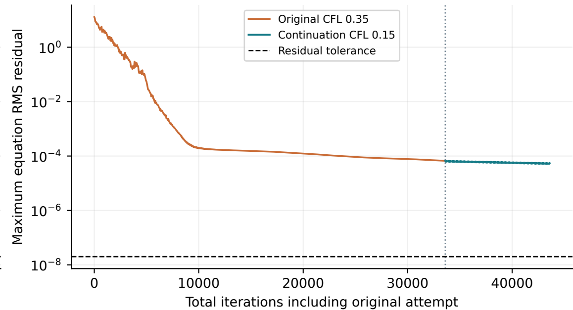
M_\infty=7.95 , N=240 : HLLC / CWENO5
