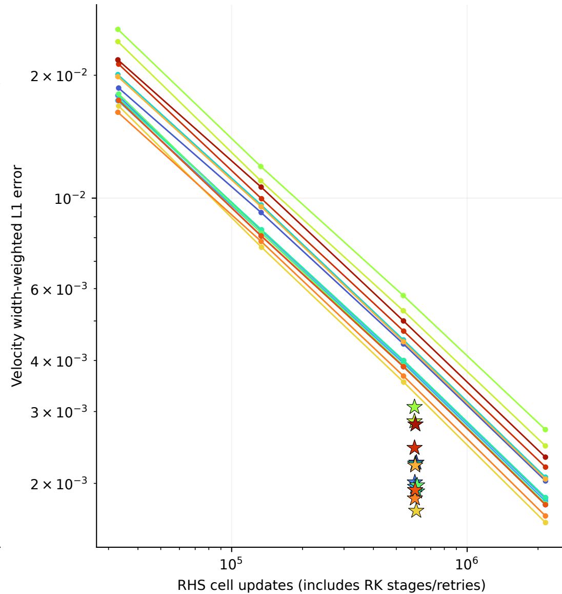
Accuracy versus numerical RHS work · stars = AMR
