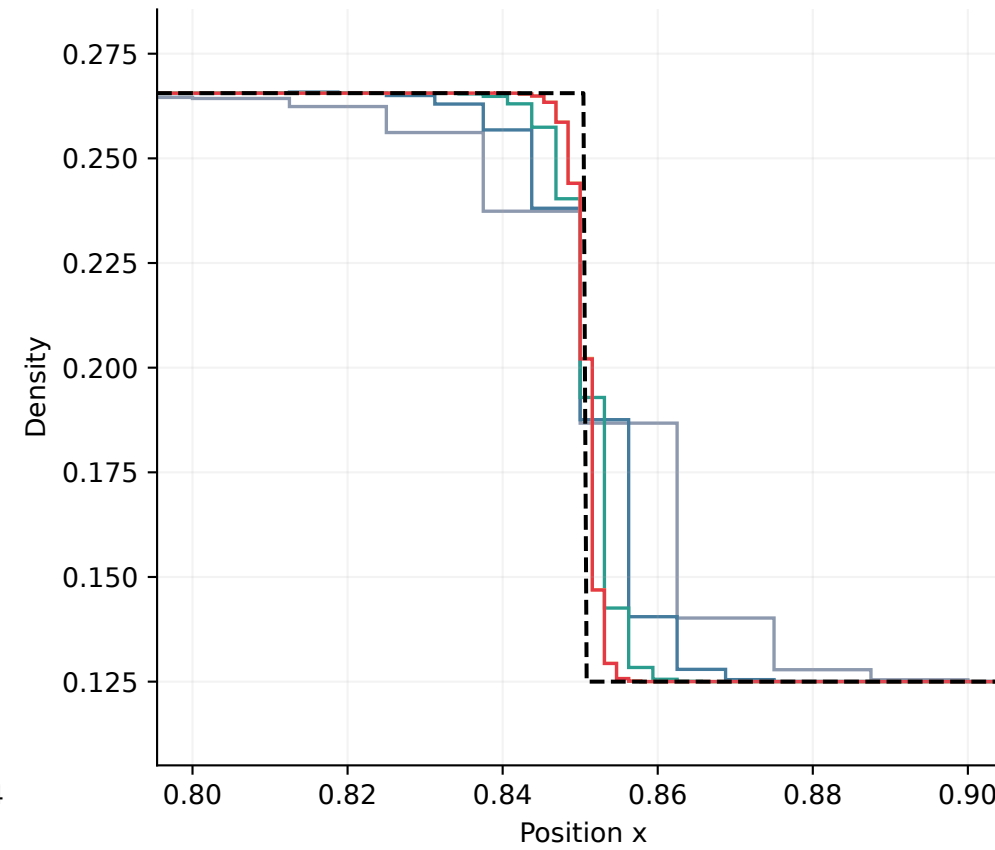
Shock detail · raw FV stairs
