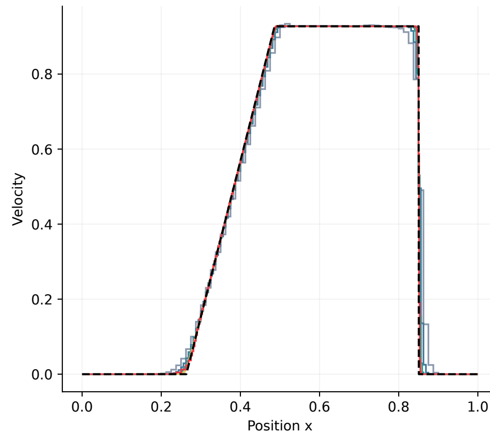
Shock detail · raw FV stairs
