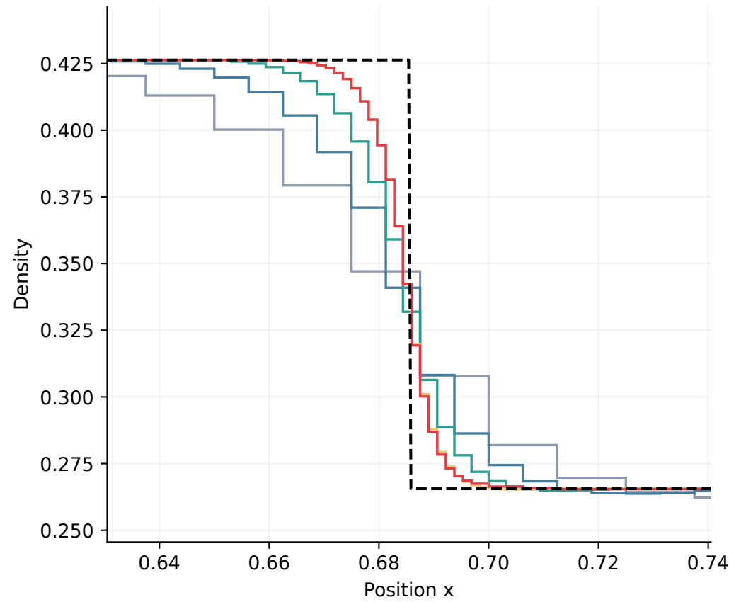
Contact detail · raw FV stairs
