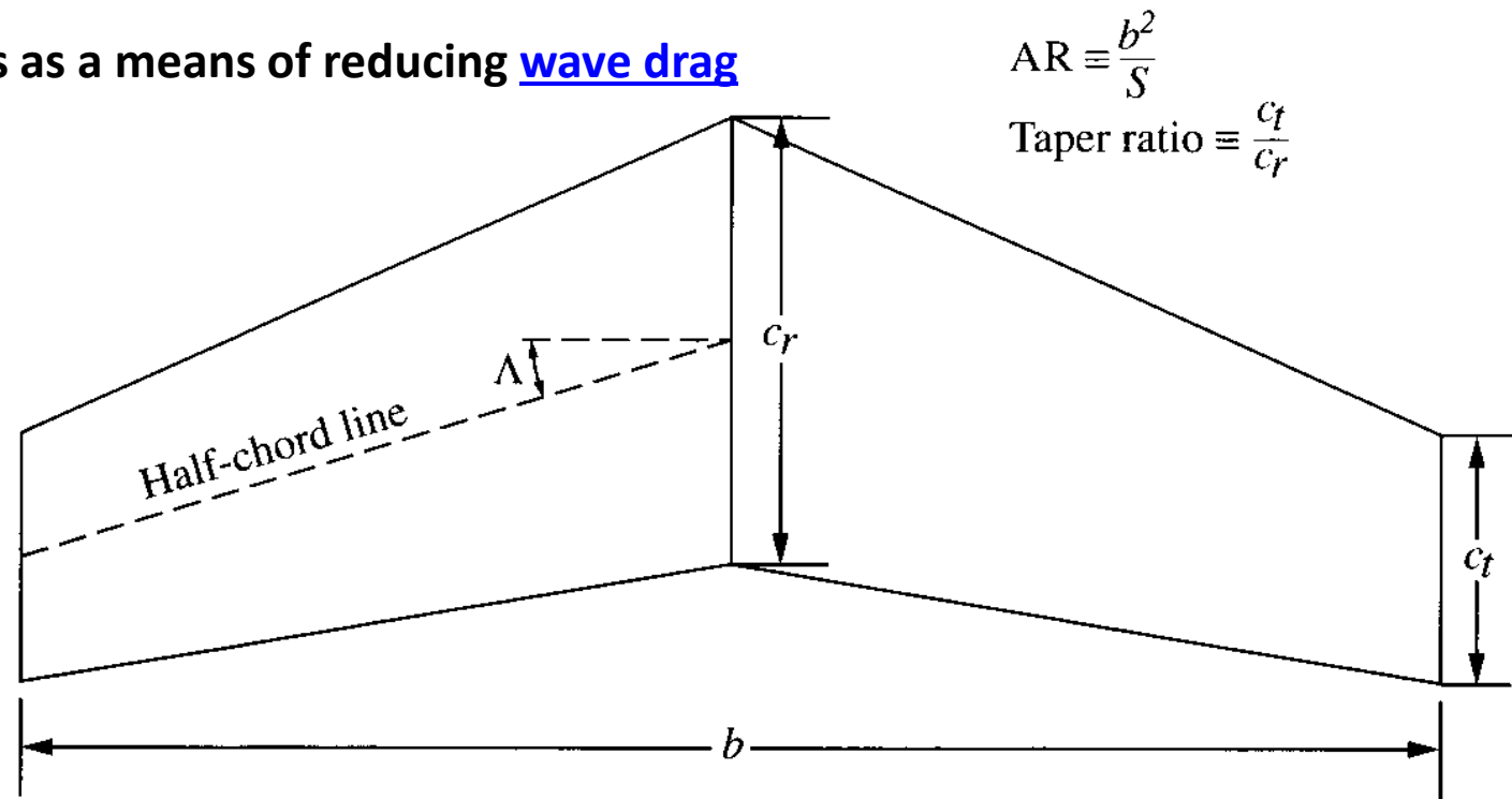
Figure 5.36 Geometry of a swept wing.
