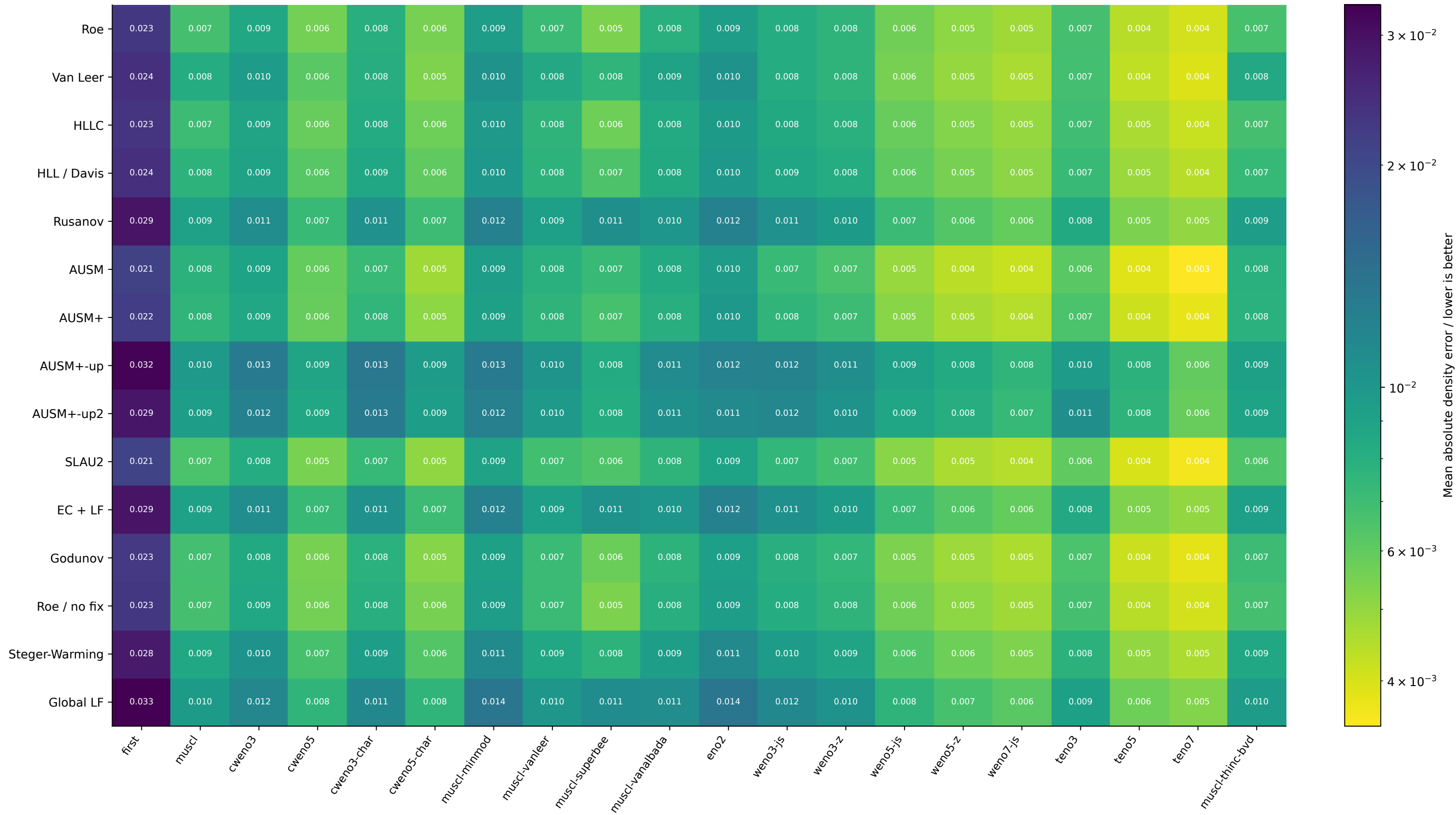
Sod · complete flux × reconstruction matrix · density L1 error
