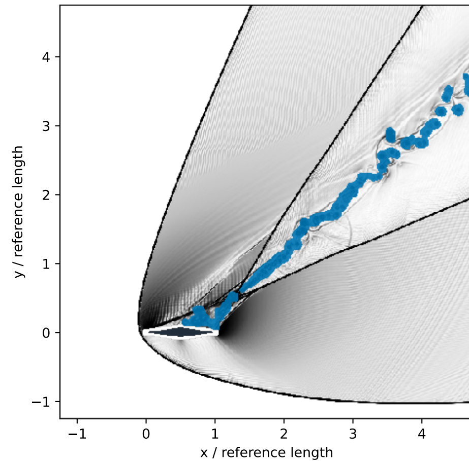
Learned vortex cores
