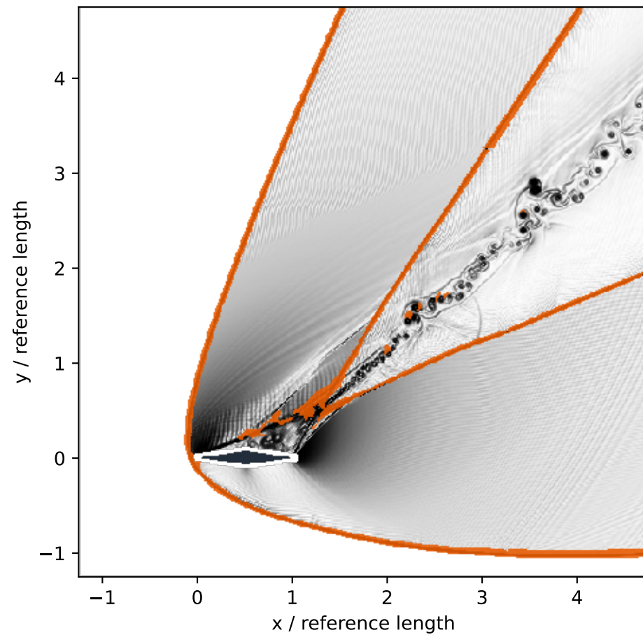
Learned shock front
