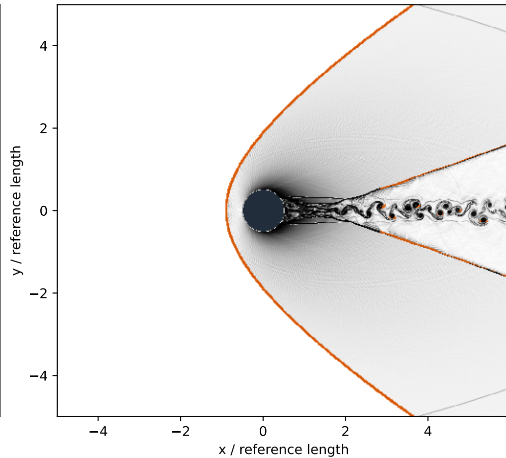
Learned shock front
