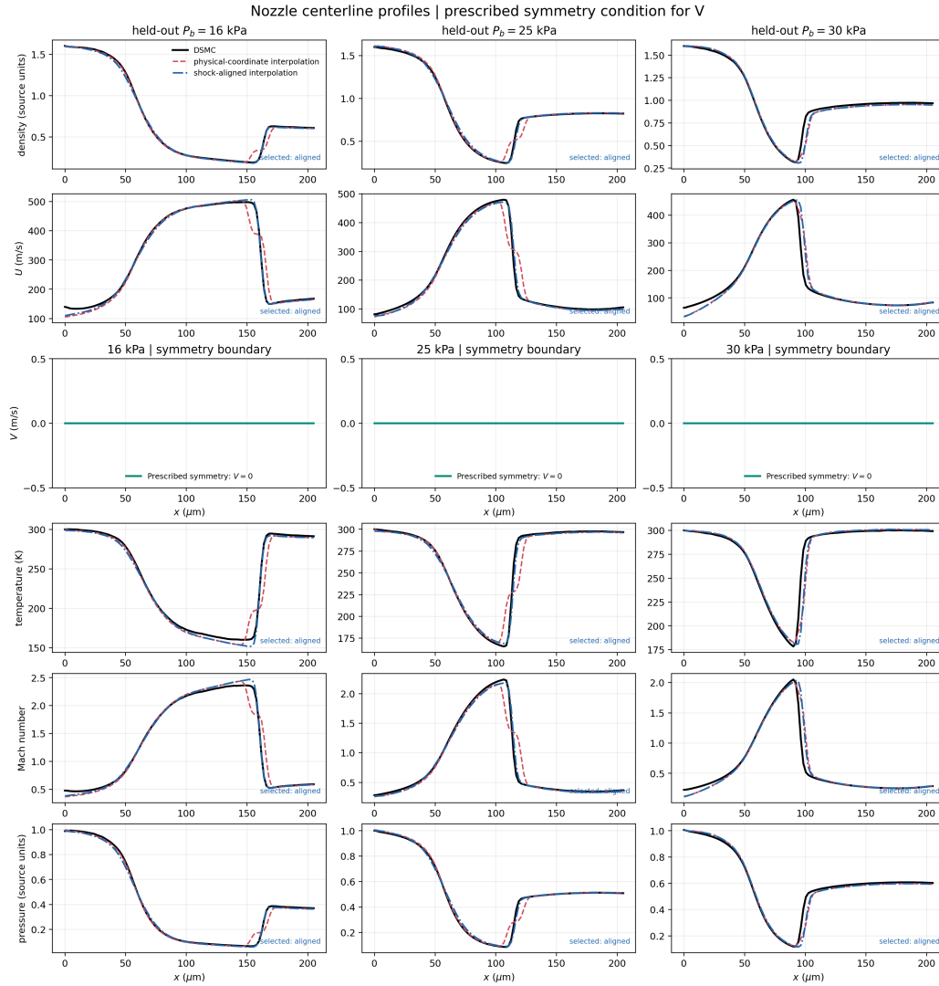
Figure 4: Centerline profiles at all three held-out back pressures. The V panels show the prescribed symmetry condition V = 0 ; they are not a learned accuracy result. Other fields compare both interpolation baselines with development-only route selection. The inconsistent raw boundary values remain in the separate symmetry audit.
