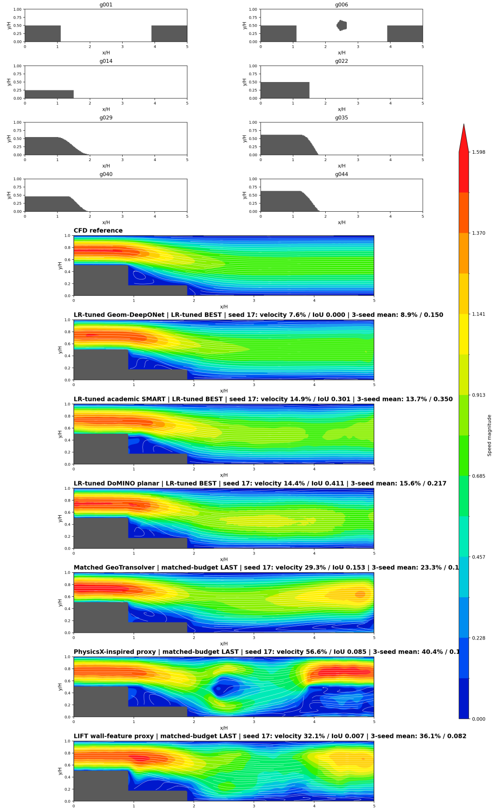
Figure 6: Extended comparison at Re=25
