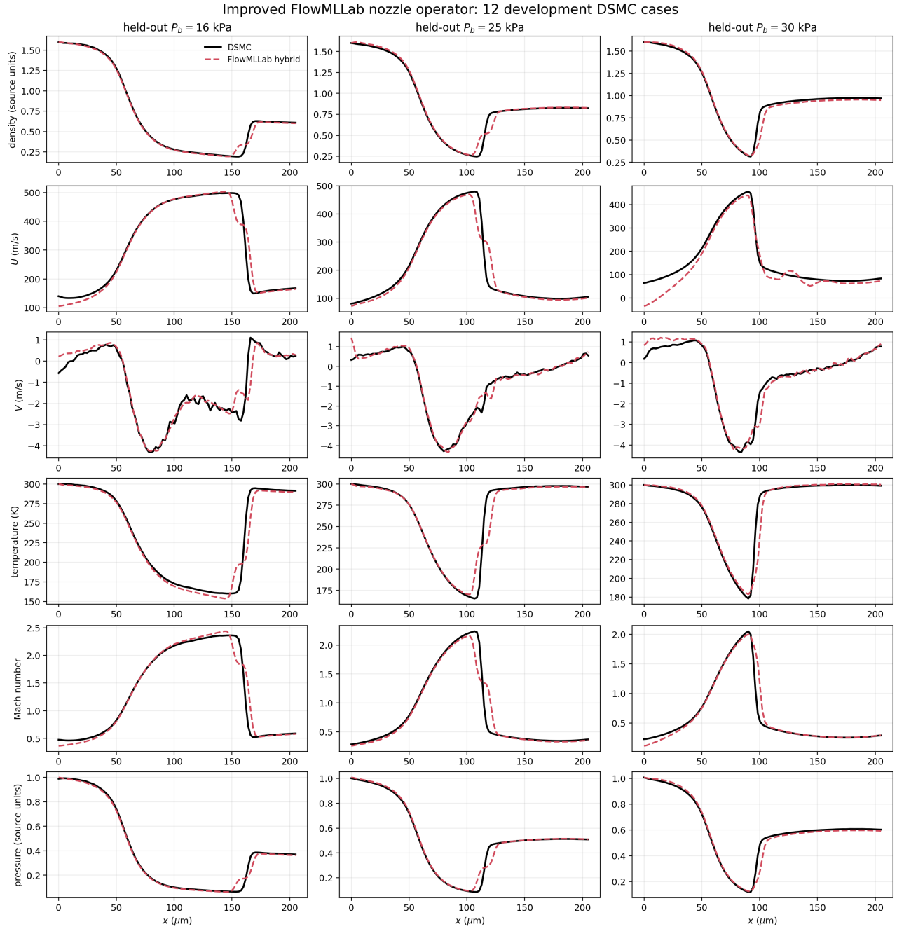
Figure 4: Centerline slices extracted from the new full-field FlowMLLab predictions for all three held-out back pressures. These curves are regenerated by qa/run_nozzle_field_validation.py .
