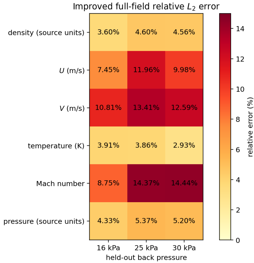
Figure 5: Full-field relative L_2 errors from the same fresh run. A single average would hide both the output dependence and the harder operating cases.
