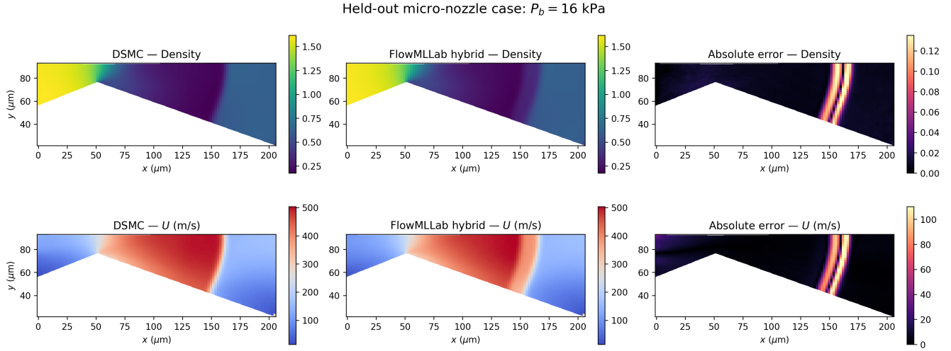
Figure 3: Improved FlowMLLab result at held-out P_b = 16 kPa. The DSMC and predicted density and U fields share color scales; error panels use absolute error. The physical axes preserve the nozzle geometry.
