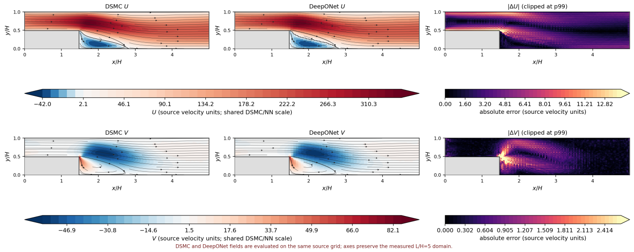
Figure 1: Micro-step rarefaction case at \text{Kn} = 0.004 : DSMC, DeepONet, and absolute velocity error, rebuilt from the pinned source fields. The solid step remains masked and the DSMC/DeepONet color limits are shared.
