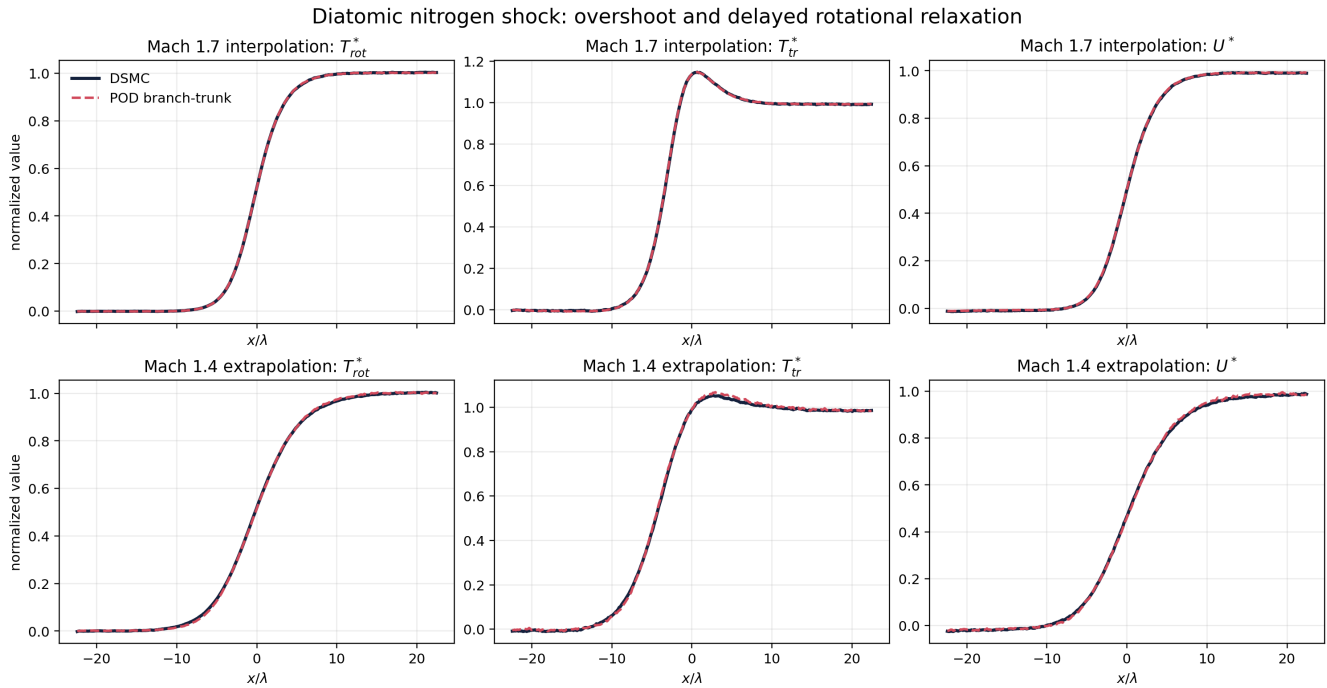
Figure 3: Reproduced diatomic nitrogen-shock profiles. The operator preserves the translational overshoot and delayed rotational relaxation.
