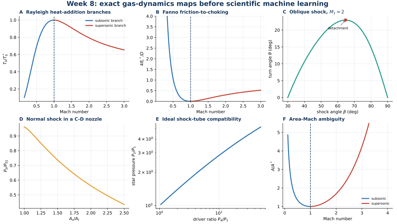
Figure 1: Exact gas-dynamics maps generated by the FlowMLLab Week-8 module. Dashed sonic lines and turning-point geometry expose the branches that an inverse model must retain.
