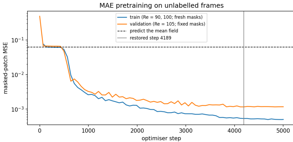
Figure 3. Masked-patch MSE during pretraining. The dashed line is the variance of v , the loss of predicting the mean field; the network sits on that plateau for a few hundred steps before it learns.
