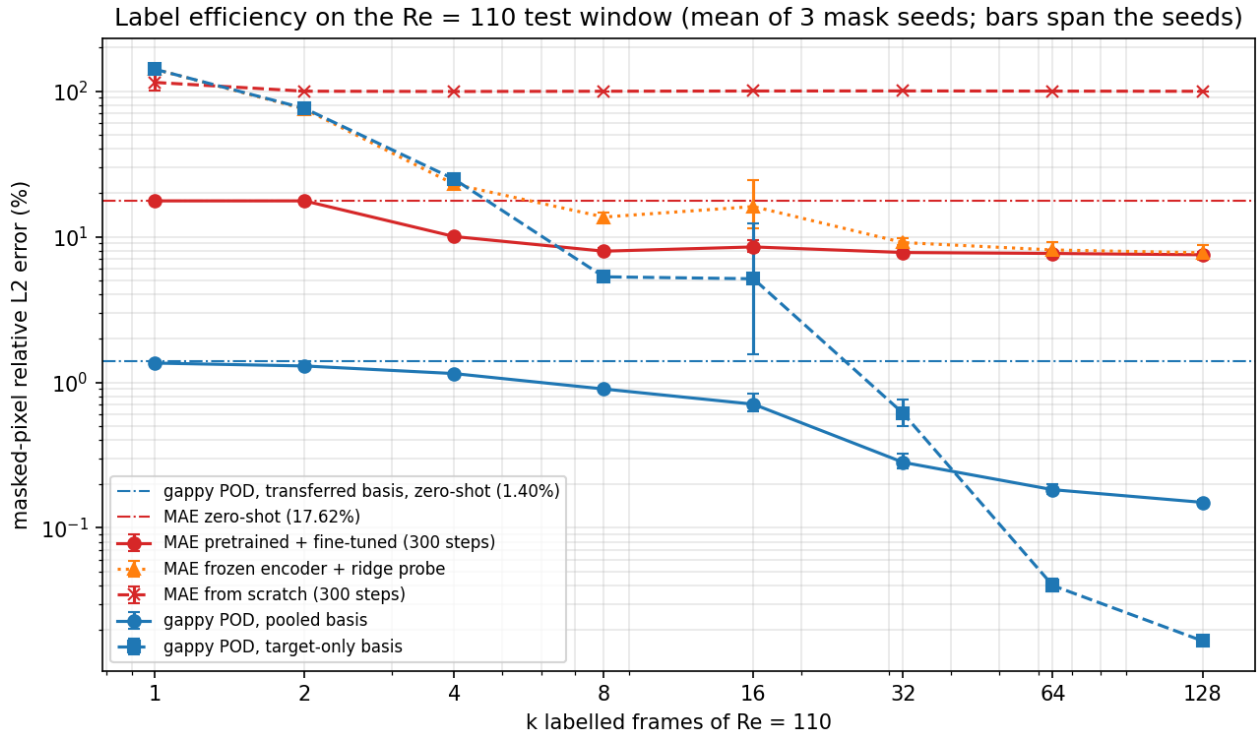
Figure 1. Masked-pixel error against the number of labelled Re = 110 frames, mean over three mask seeds of one trajectory; the bars span the three seeds. Horizontal lines are the zero-shot methods.
