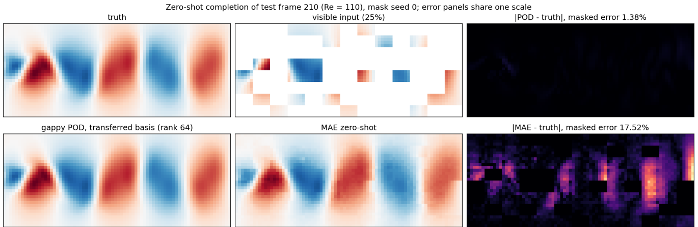
Figure 2. Zero-shot completion of test frame 210 (mask seed 0): truth, the 25% of pixels every method receives, and the two reconstructions with absolute-error maps on one scale.
