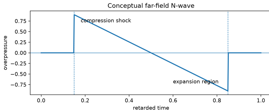
Figure 2: Conceptual N-wave. This is a teaching schematic, not a waveform computed in Week 16.
