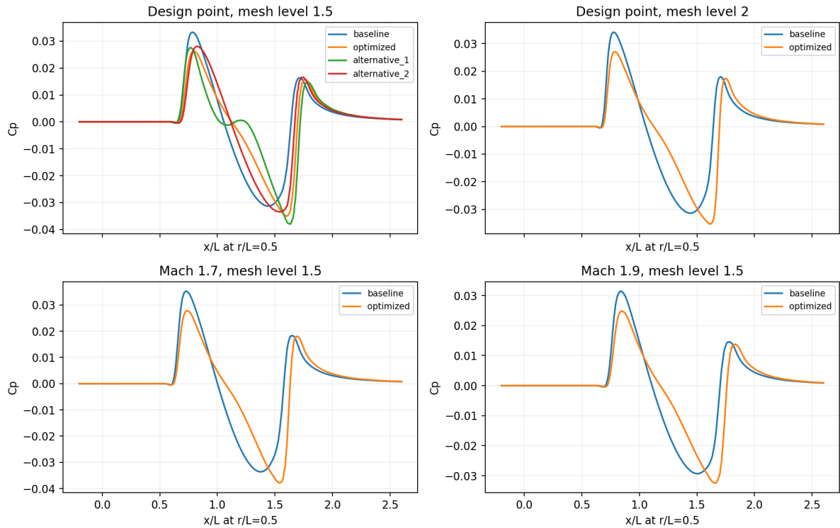
Figure 12: Independent SU2 8.0.1 recomputation of the retained candidate, including design-point mesh comparison and off-design Mach-number checks.
