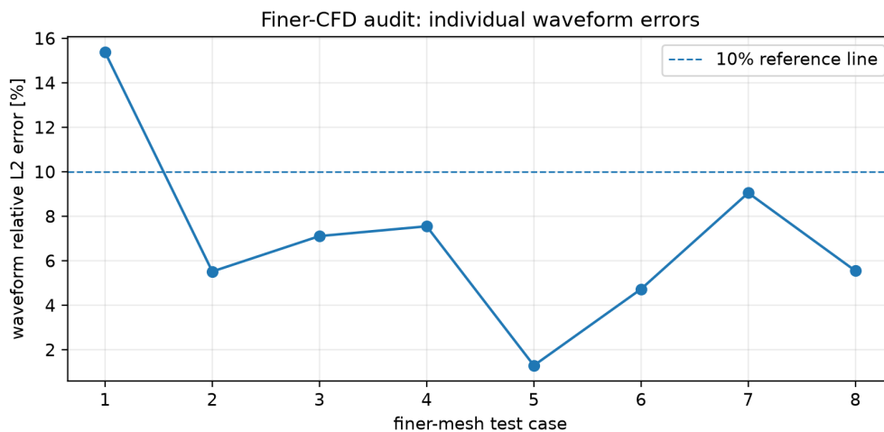
Figure 11: Individual waveform errors against the eight finer CFD references. Aggregate acceptance does not mean every case lies below 10%.
