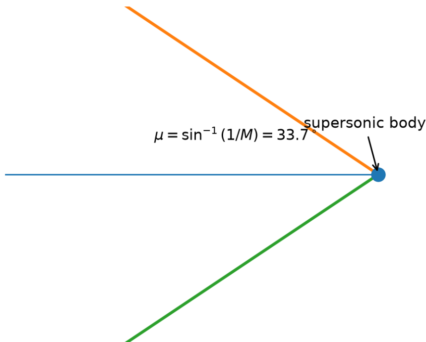
Figure 1: Schematic Mach cone for M = 1.8 . The angle is set by kinematics; finite-amplitude compression waves can steepen into shocks.
