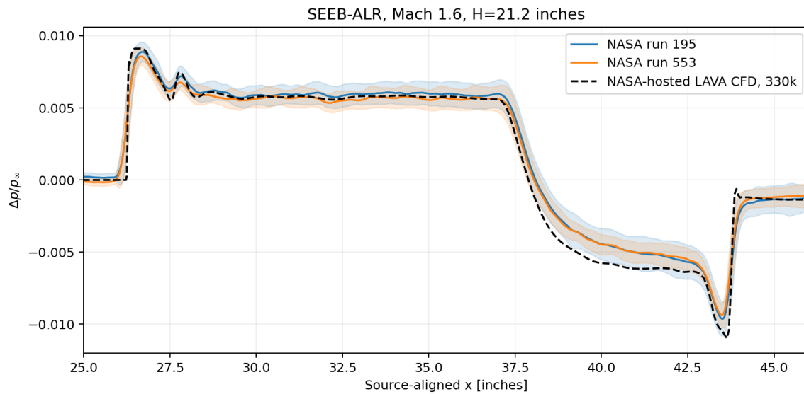
Figure 13: Retained NASA SEEB-ALR reference comparison. The LAVA result is an independent numerical solution, not an exact answer. Experimental agreement and solver-to-solver agreement answer different questions.
