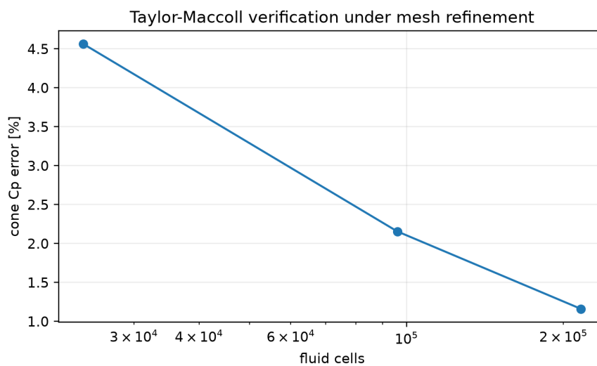
Figure 5: Taylor–Maccoll verification. Refinement reduces the analytical cone-pressure error; the finest result is within the declared 3% criterion.
