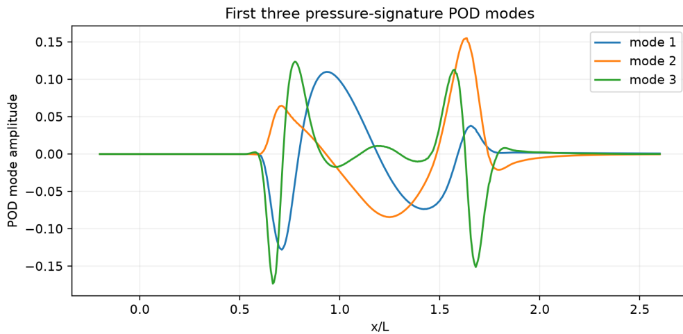
Figure 9: The first three training pressure modes. The modes encode coherent changes in amplitude and wave position across the geometry family.
