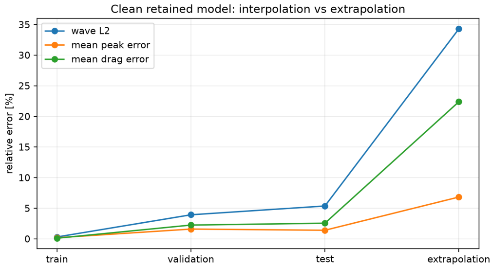
Figure 10: Retained clean-label model errors across the frozen splits. Extrapolation degrades sharply even though interpolation errors remain modest.
