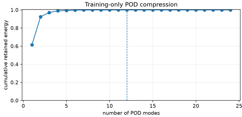
Figure 8: Cumulative POD energy from the training set only.
