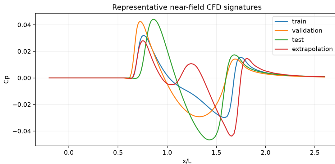
Figure 7: Representative accepted CFD pressure signatures from each split. Shock location and amplitude both change with geometry.
