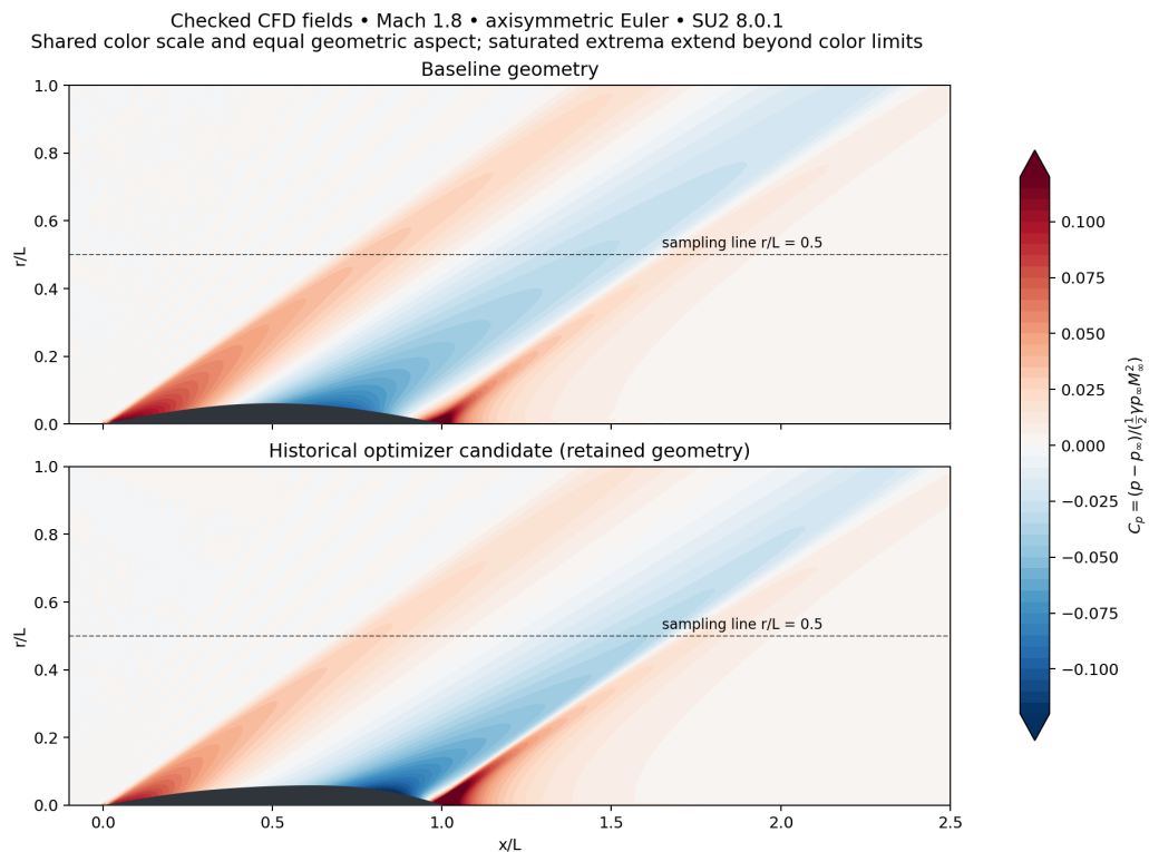
Figure 4: Accepted SU2 8.0.1 pressure fields for the baseline and retained optimizer geometry. The dashed line is the primary sampling location r/L = 0.5 . Shared color limits make redistribution of the compression/expansion field directly visible.
