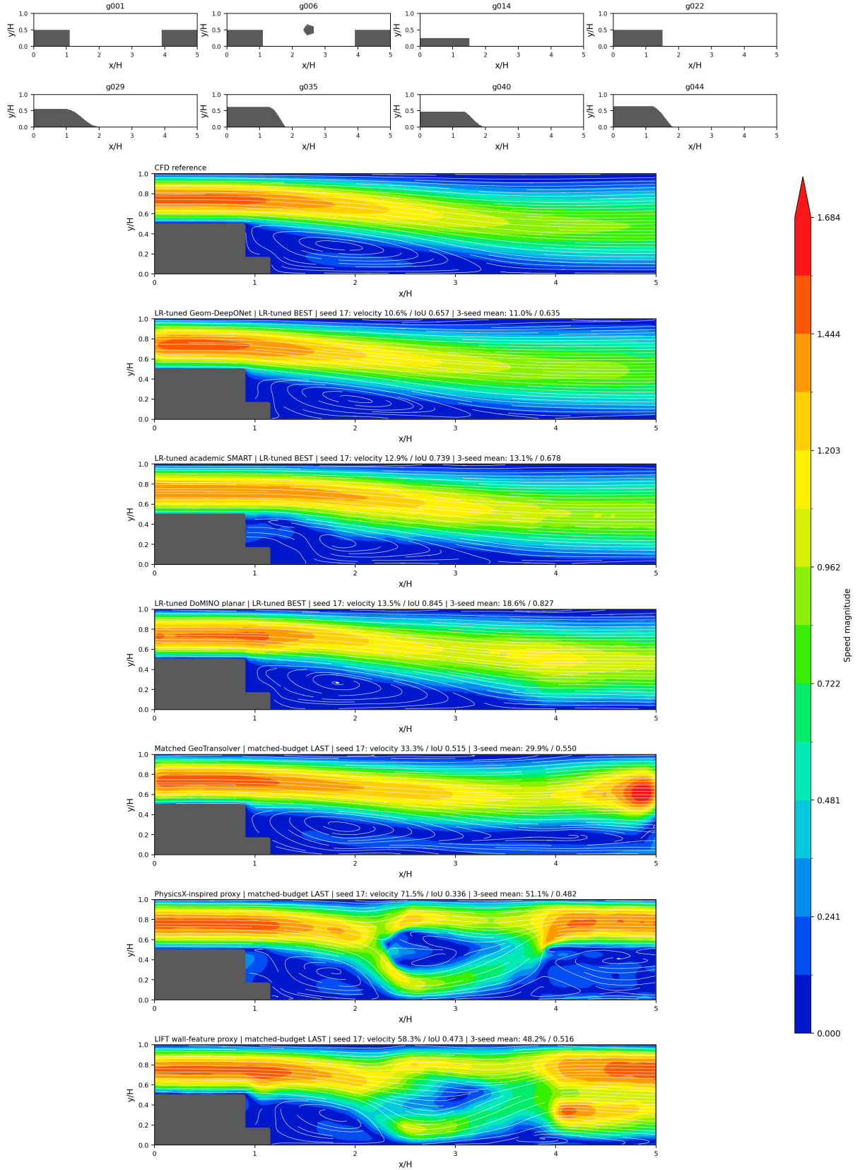
Figure 8: Extended comparison at Re=100
