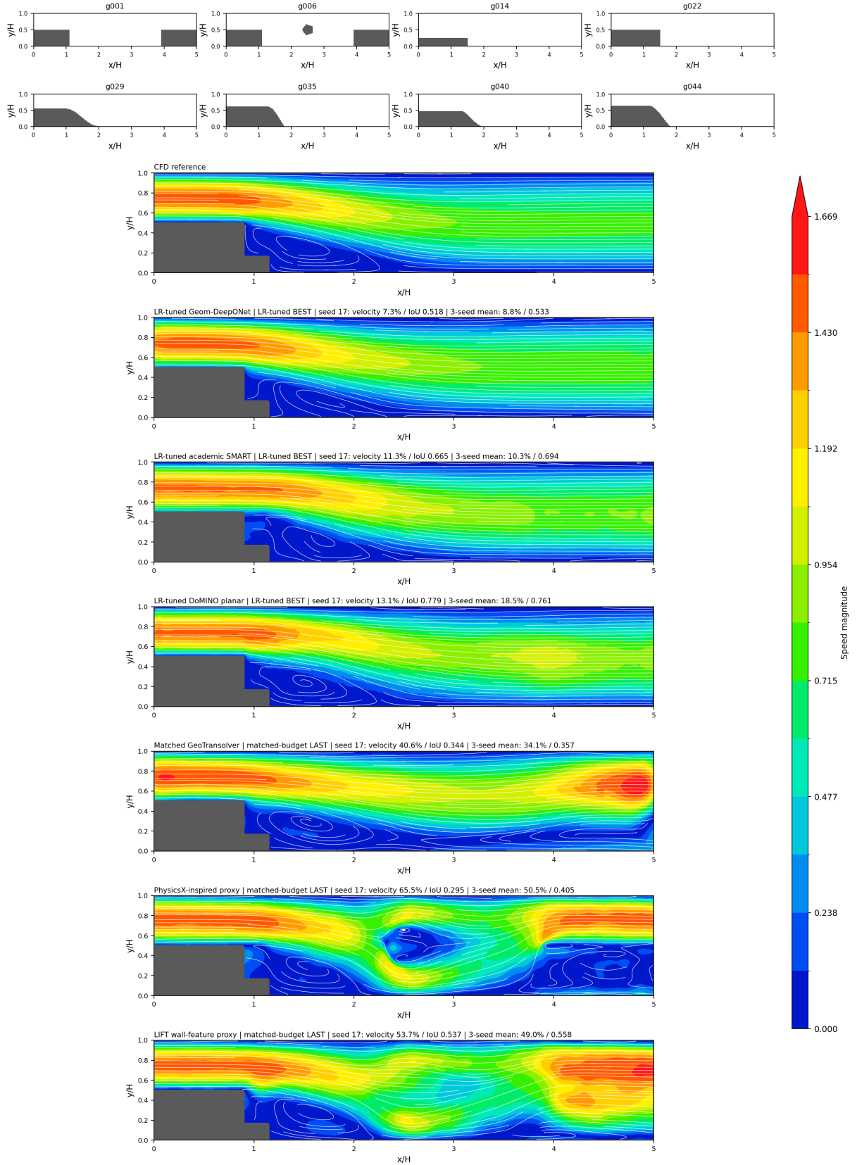
Figure 7: Extended comparison at Re=50
