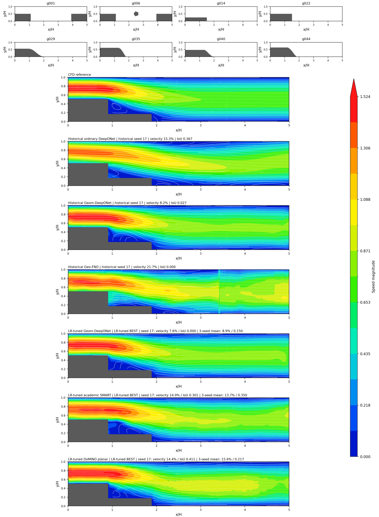
Figure 3: Core comparison at Re=25
