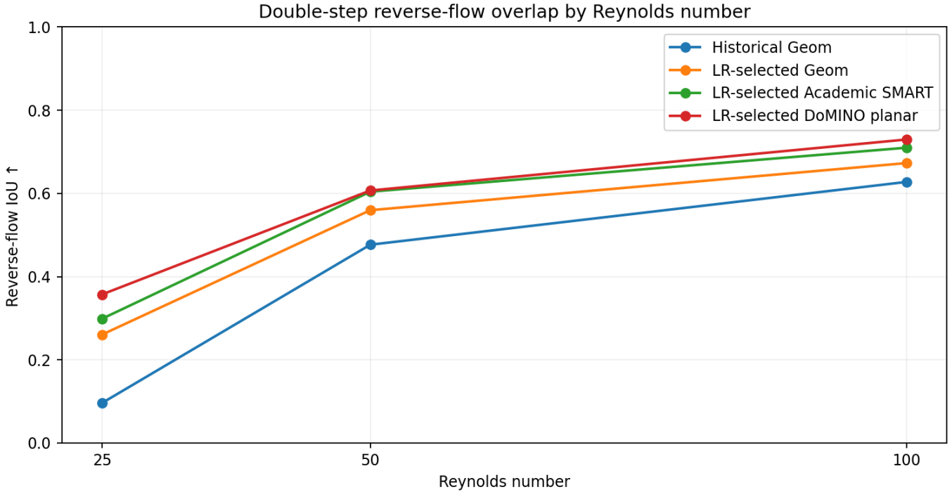
Figure 2: Reynolds-stratified reverse-flow IoU
