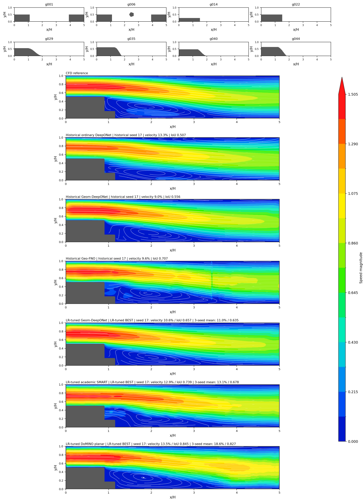
Figure 5: Core comparison at Re=100
