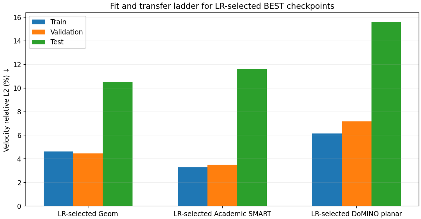
Figure 9: Train-validation-test velocity ladder
