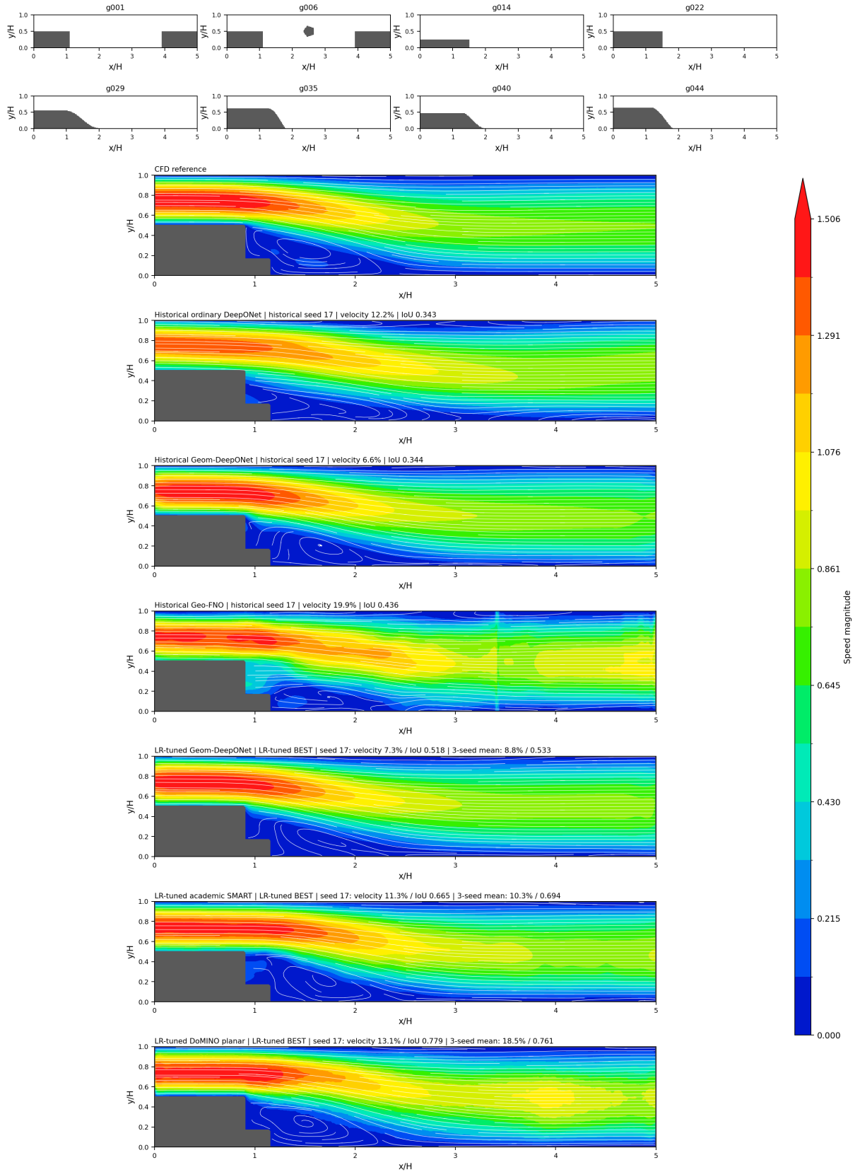
Figure 4: Core comparison at Re=50
