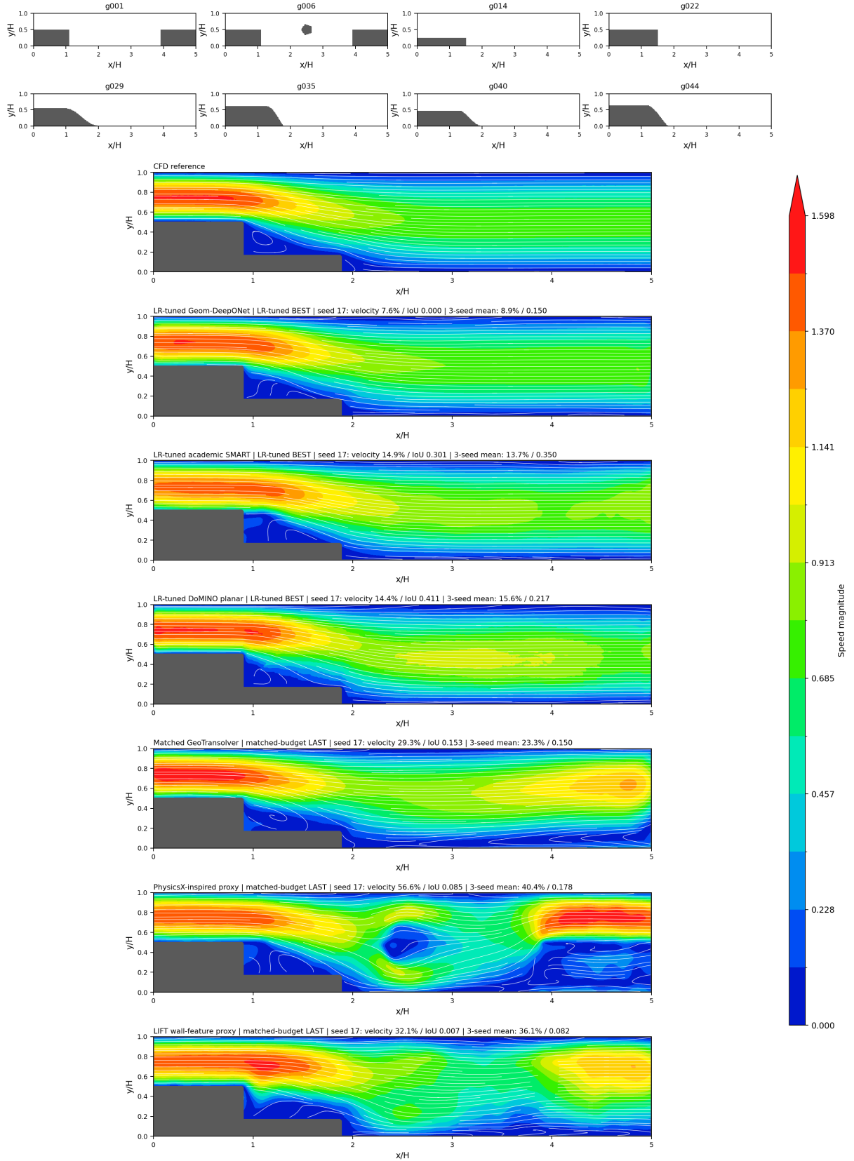
Figure 6: Extended comparison at Re=25
