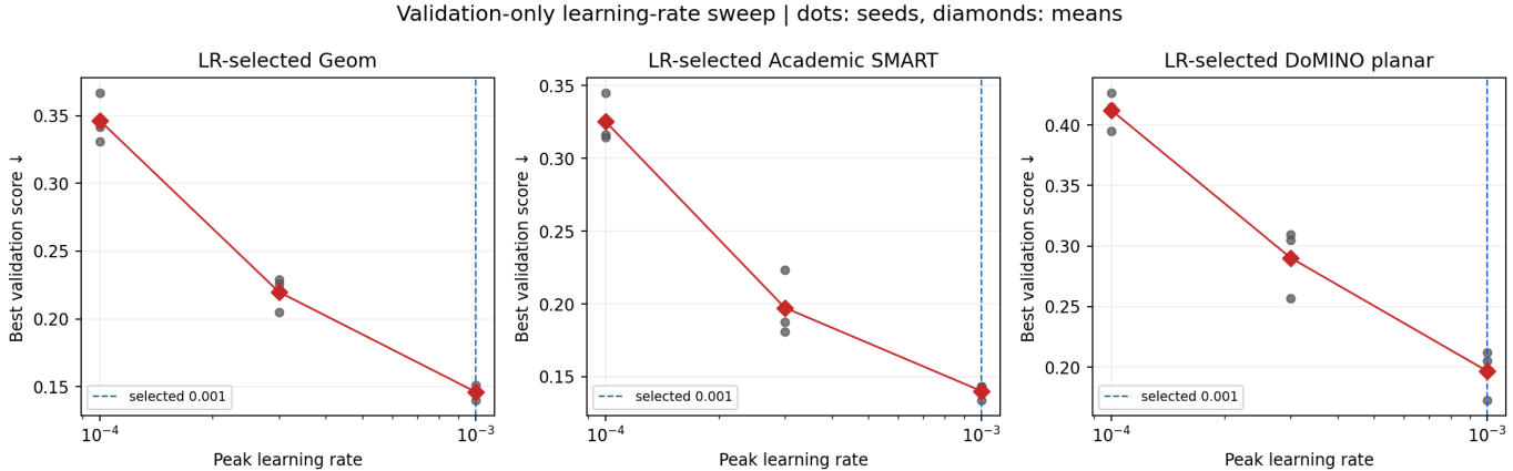
Figure 1: Validation-only learning-rate sweep
