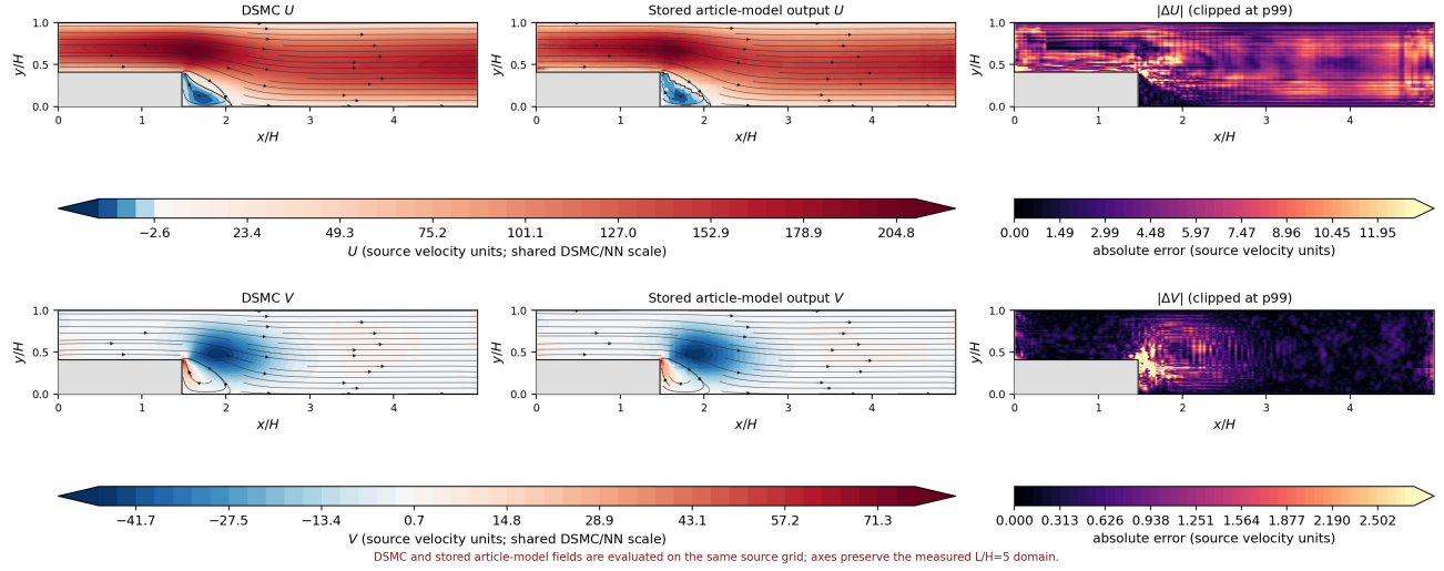
Figure 2: Article height-variation case H44: DSMC and stored target-assisted reconstruction, rebuilt on the source grid. The article-model input includes a local patch from the target DSMC field. Reverse-flow IoU and reattachment length complement the vector relative L_2 value.
