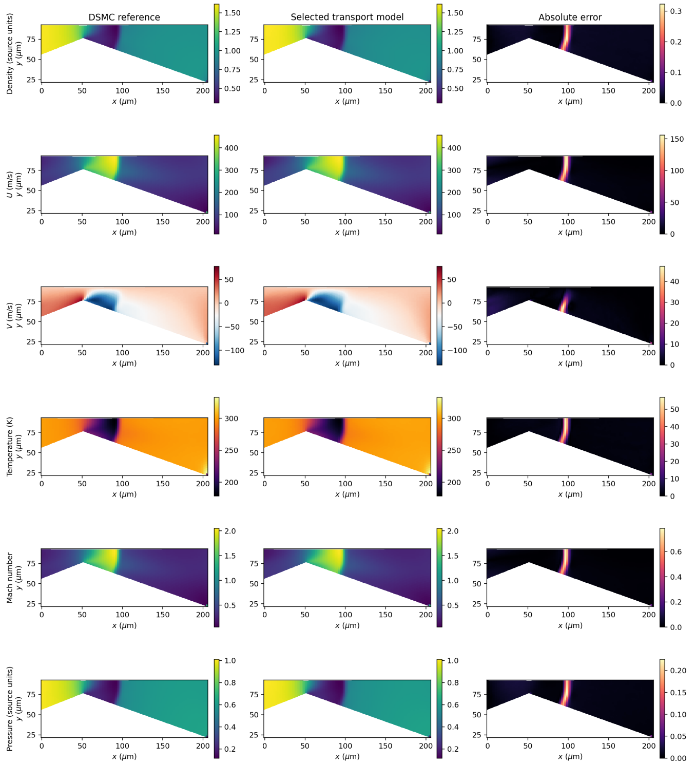
Micro-nozzle at 30 kPa | all six physical fields
