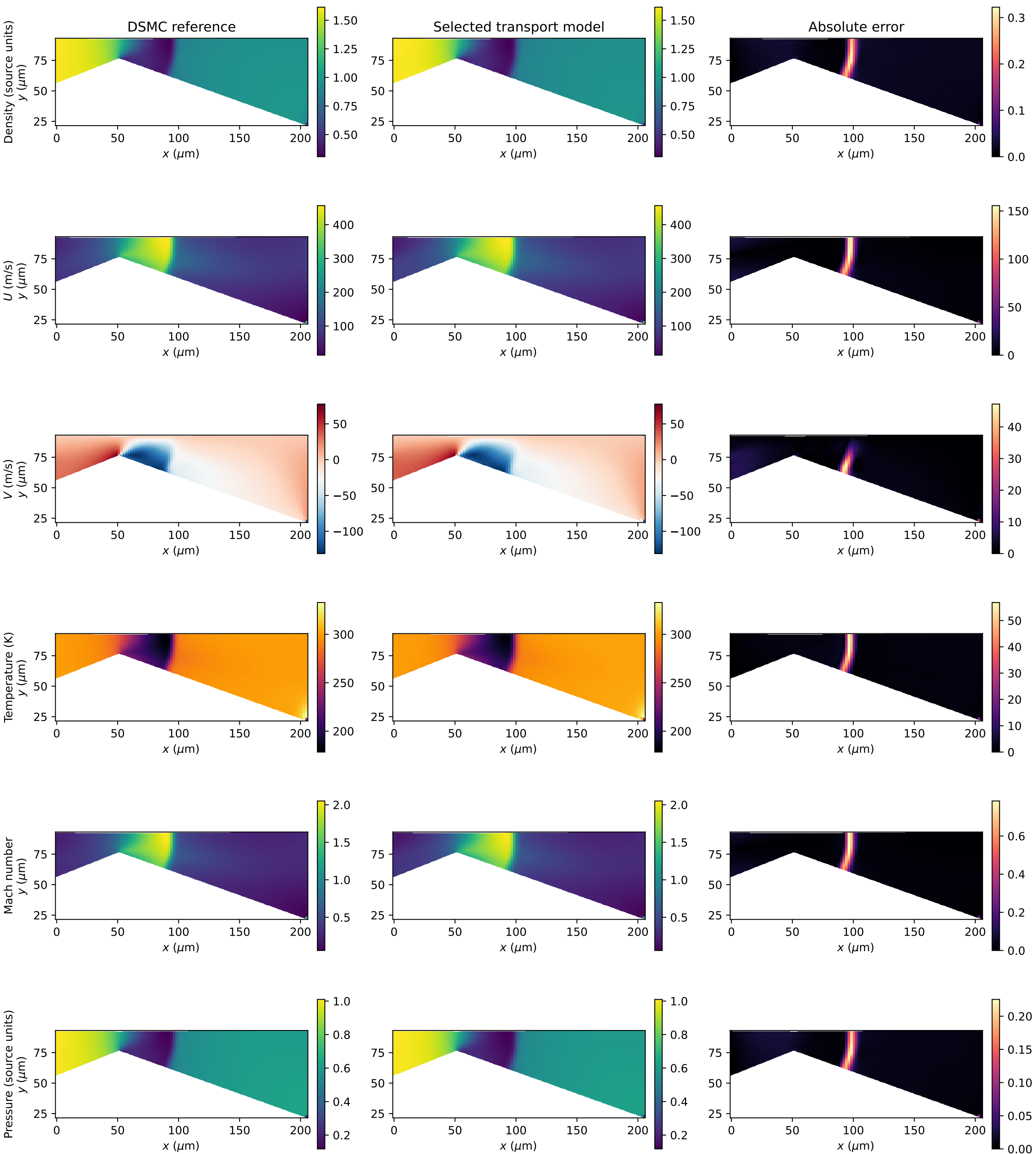
Micro-nozzle at 30 kPa | all six physical fields
