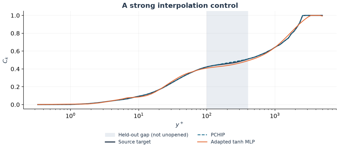
Figure 5. PCHIP and the separately labeled tanh-MLP control over the historically inspected held-out interval.
