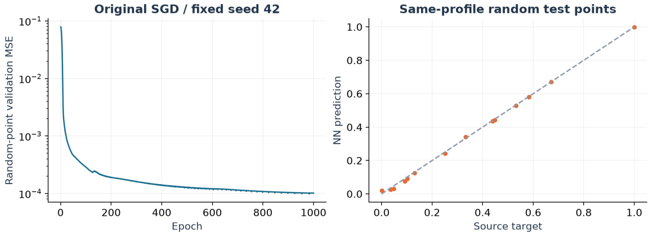
Figure 4. Original c_k regression protocol with an explicit initialization seed. Random-point accuracy is not whole-case transfer.
