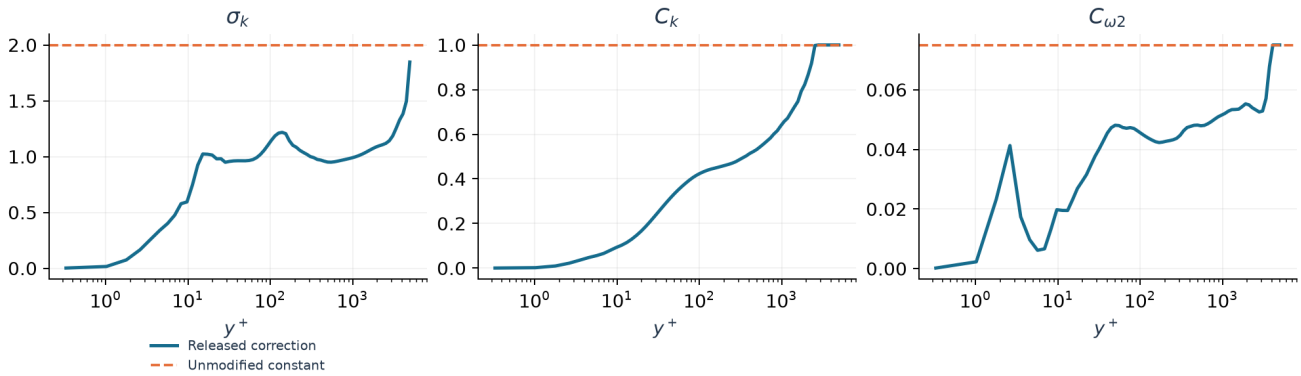
Figure 3. Released spatial correction coefficients and unmodified model constants.
