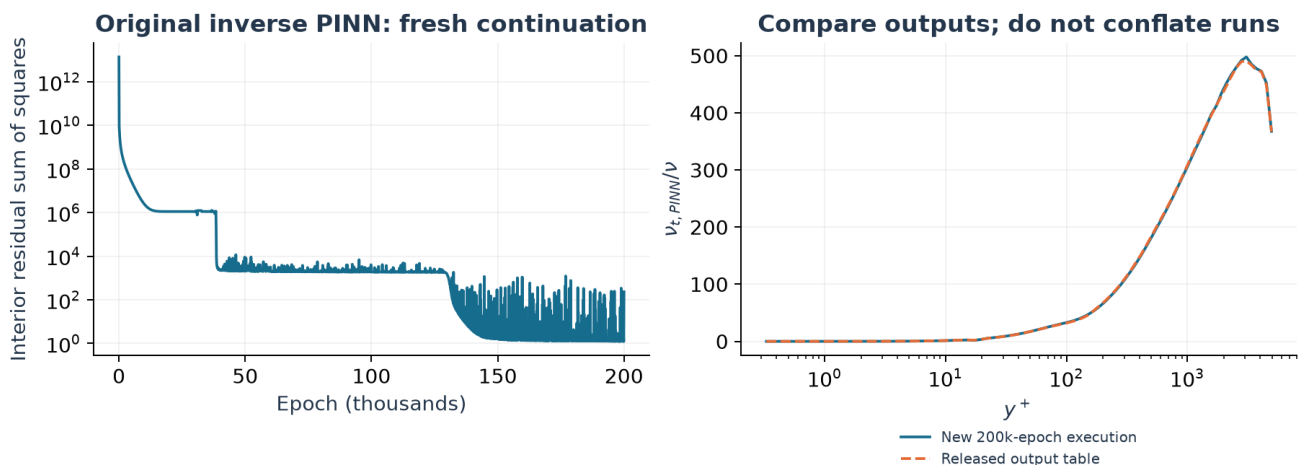
Figure 7. Fresh 200,000-epoch checkpoint continuation and the released diffusion profile. Minimum and final loss are distinct.
