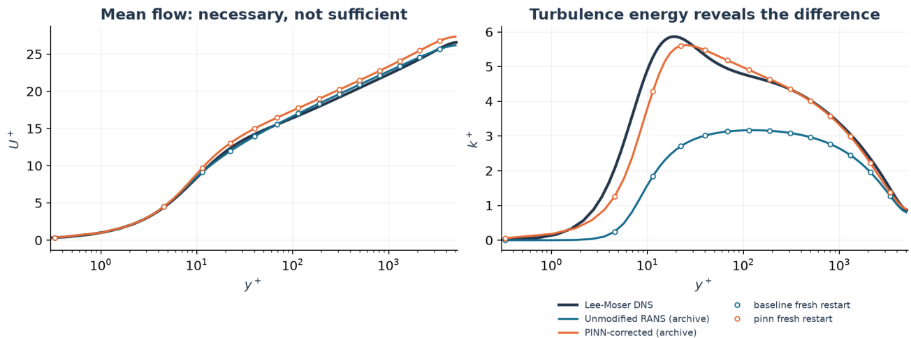
Figure 1. Classical and table-based PINN profiles against Lee-Moser DNS. Markers are fresh restarted solves, not a verified reproduction of the final PINN-NN curves in Figure 8 of the paper.
