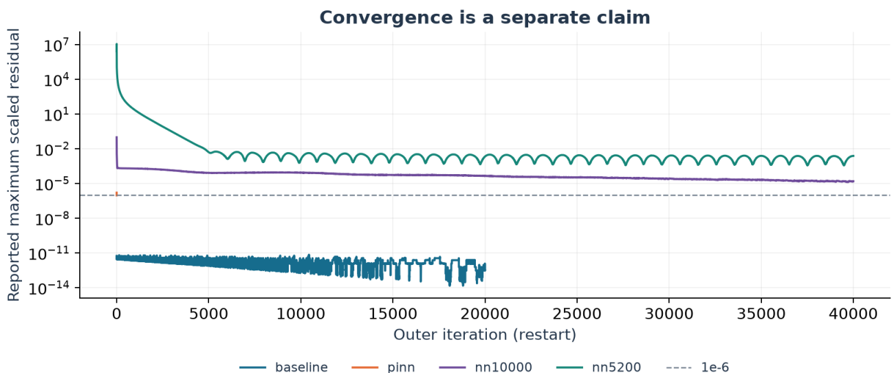
Figure 6. Source-solver residuals. NN5200 is an assembled case; neither NN run meets the requested 1e-6 criterion.
