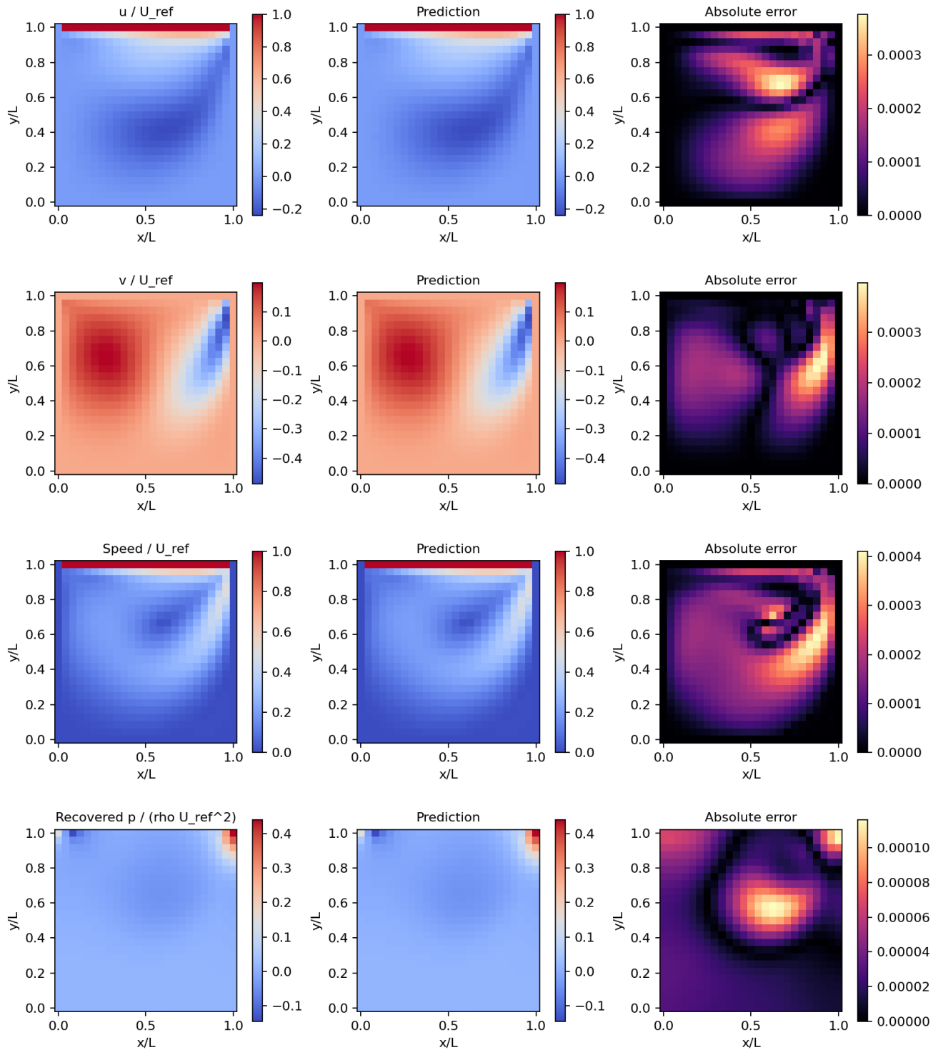
Constant lid | first held-out case | Re = 378.4 Left: NS reference | center: Stokes + neural correction | right: error
