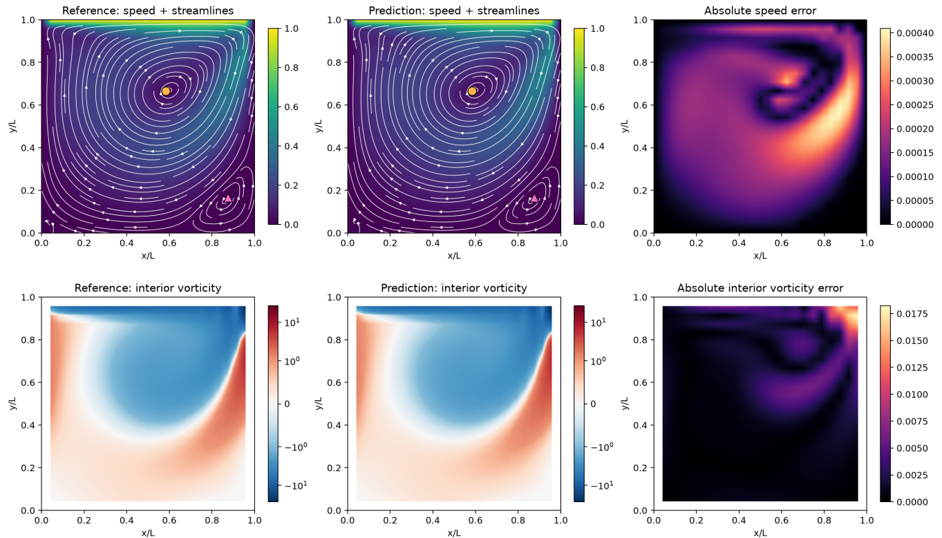
Constant lid | first retained test case | Re = 378.4 Navier-Stokes reference vs Stokes-corrected prediction
