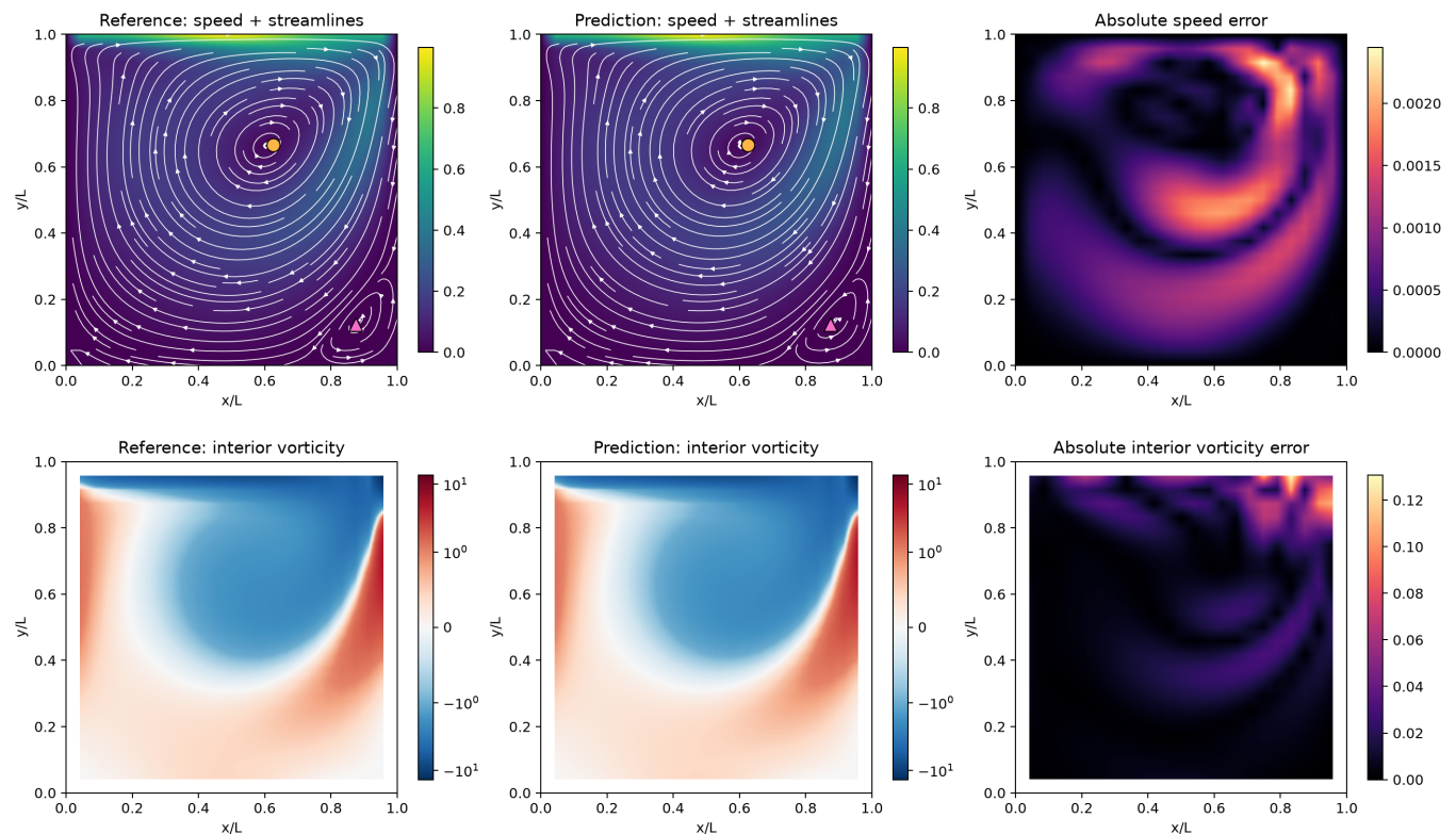
Diverse lid | first retained test case | Re = 378.4 Navier-Stokes reference vs Stokes-corrected prediction
