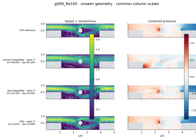
Figure 4. Unseen geometry g009 at Re=100: CFD, ordinary DeepONet, Geo-DeepONet, and FNO in rows. Row labels report seed-17 velocity and centered-pressure errors; ordinary DeepONet is markedly worse.
