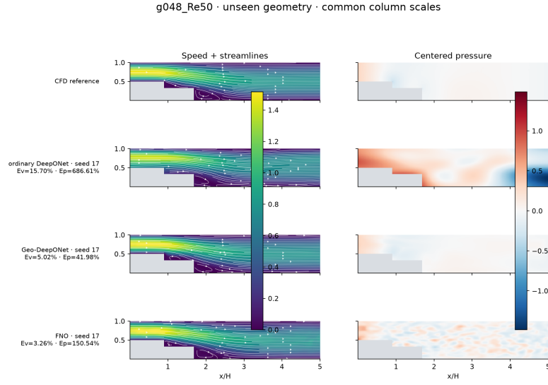
Figure 5. Unseen geometry g048 at Re=50: the fixed-domain DeepONet is shown beside geometry-aware and spectral operators, with seed-17 errors printed in each row.
