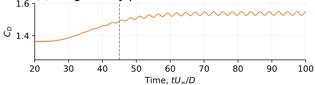
(c) Drag history | D40
