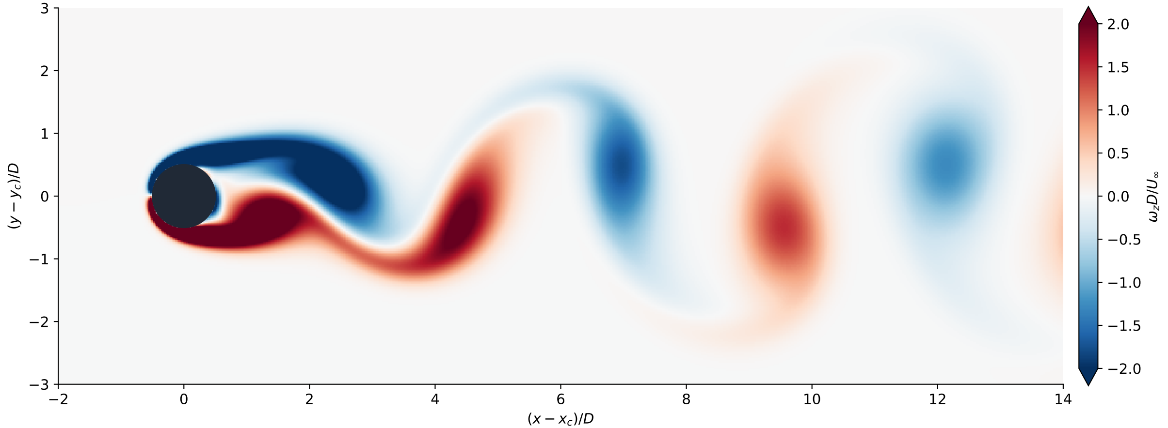
(a) Alternating vortex wake | D40, final field at tU/D = 100
