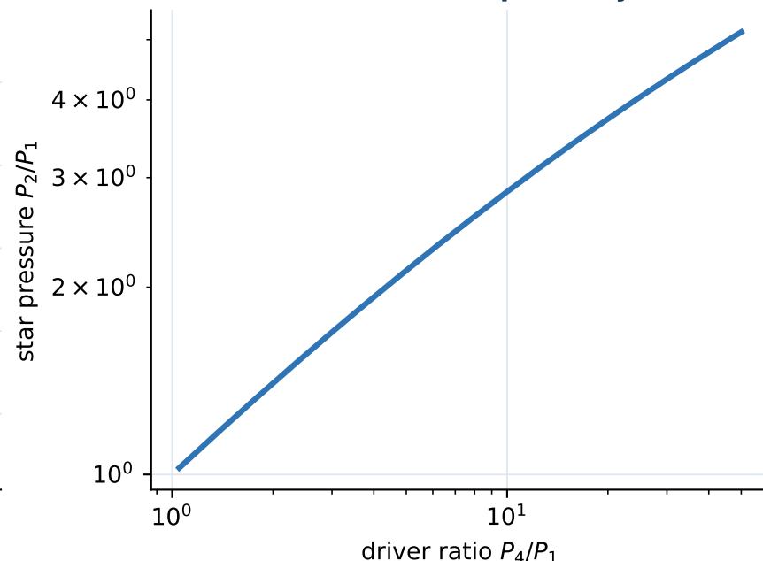
E Ideal shock-tube compatibility
