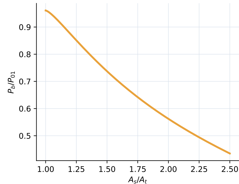
D Normal shock in a C-D nozzle
