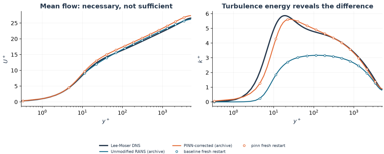
Figure 1. Classical and table-based PINN profiles against Lee-Moser DNS. Markers are fresh restarted solves, not a verified reproduction of the final PINN-NN curves in Figure 8 of the paper.
