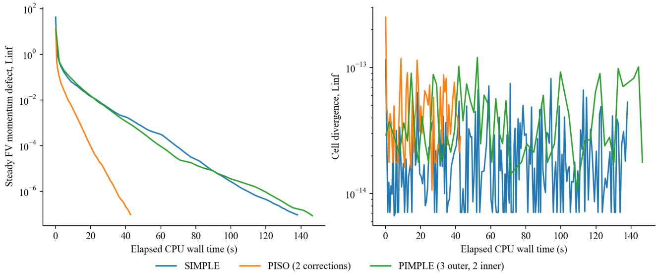
Coupling convergence: one measured local CPU solve per method
