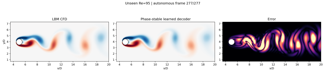
Figure 6: Fresh unseen Re = 95 field comparison after autonomous evolution. The axes use equal physical scale, so the analytical cylinder is displayed as a circle. The error panel has its own colour scale.
