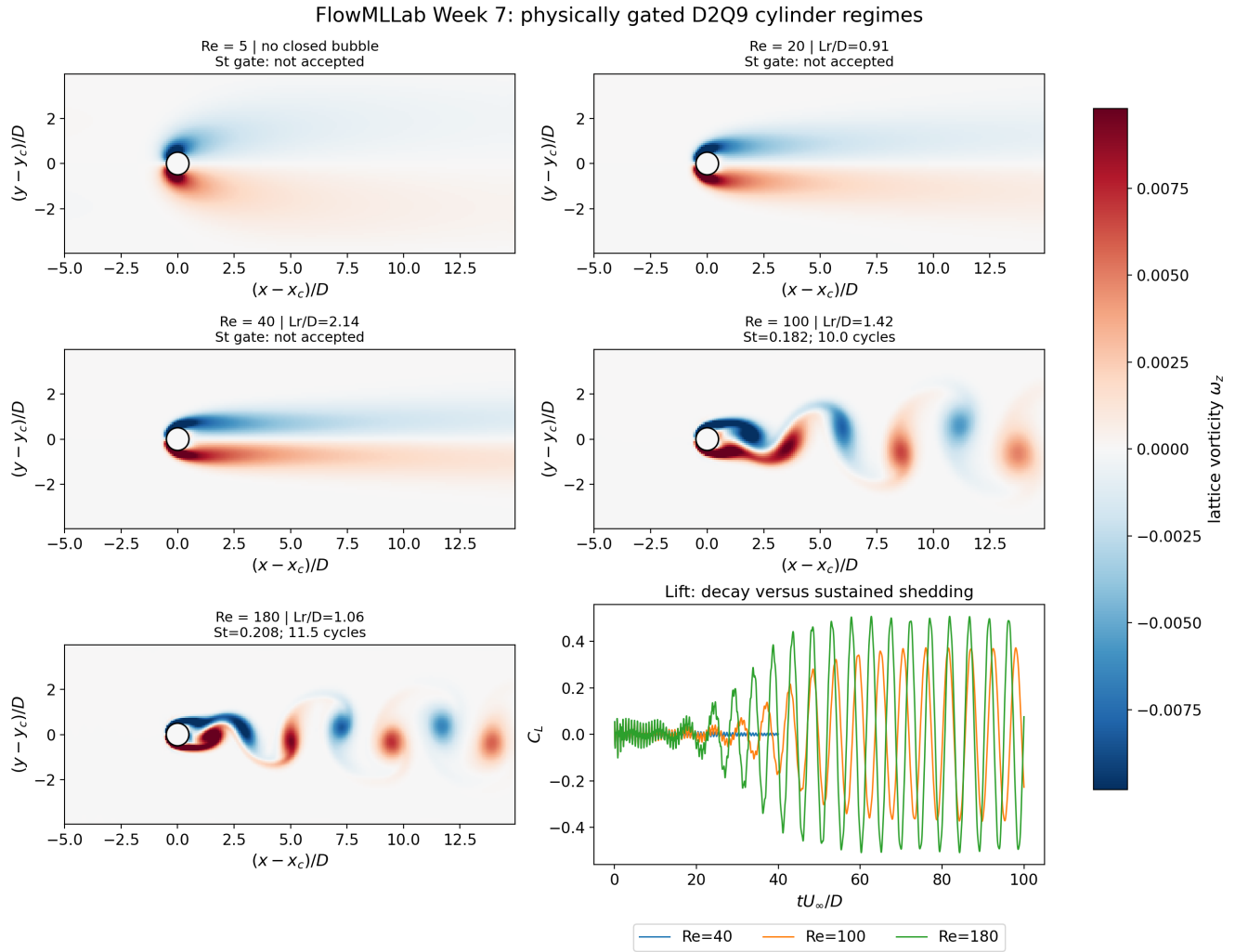
Figure 1: Retained D2Q9 regime evidence. The contour, force history, frequency quality flags, and time-mean recirculation length are interpreted together.
