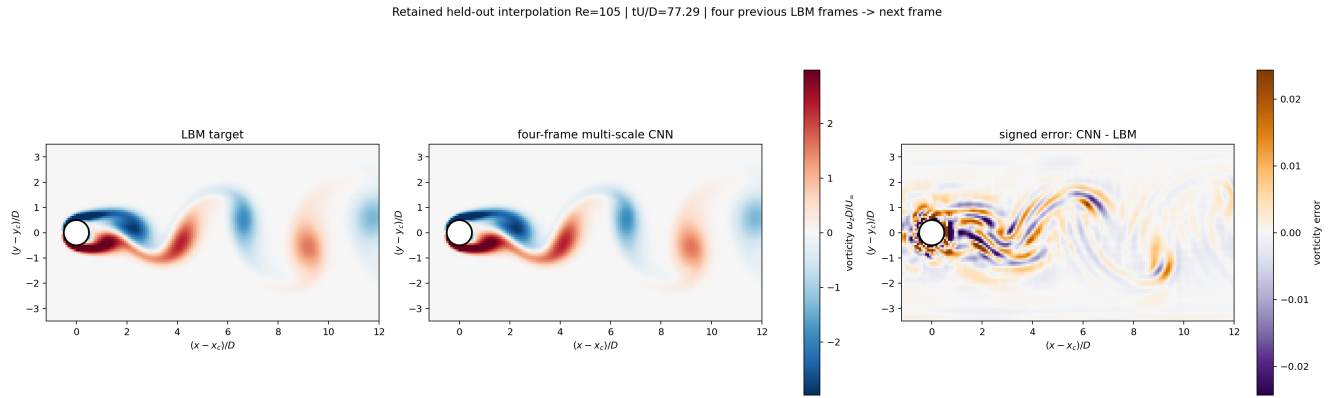
Figure 2: Retained Re = 105 one-step interpolation. Each target uses four true prior LBM fields. Identical colour limits are used for LBM and CNN; the signed error has its own much narrower scale.
