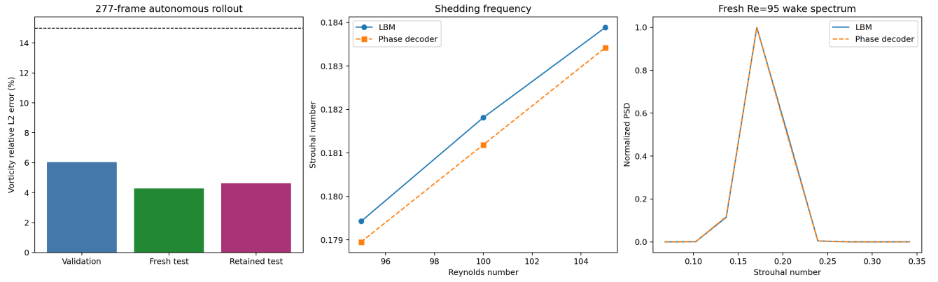
Figure 5: Leakage-controlled long-horizon evidence. Left: global vorticity error against the predeclared gate. Centre: LBM and decoder Strouhal numbers. Right: overlapping fresh-test wake spectra at Re = 95 .
