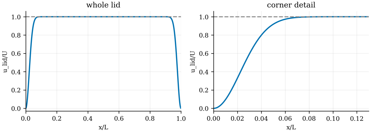
Figure 2. Smooth lid profile used by the hard lifting (blue) versus an ideal unit lid (gray). The regularization width is part of the boundary-value problem.
