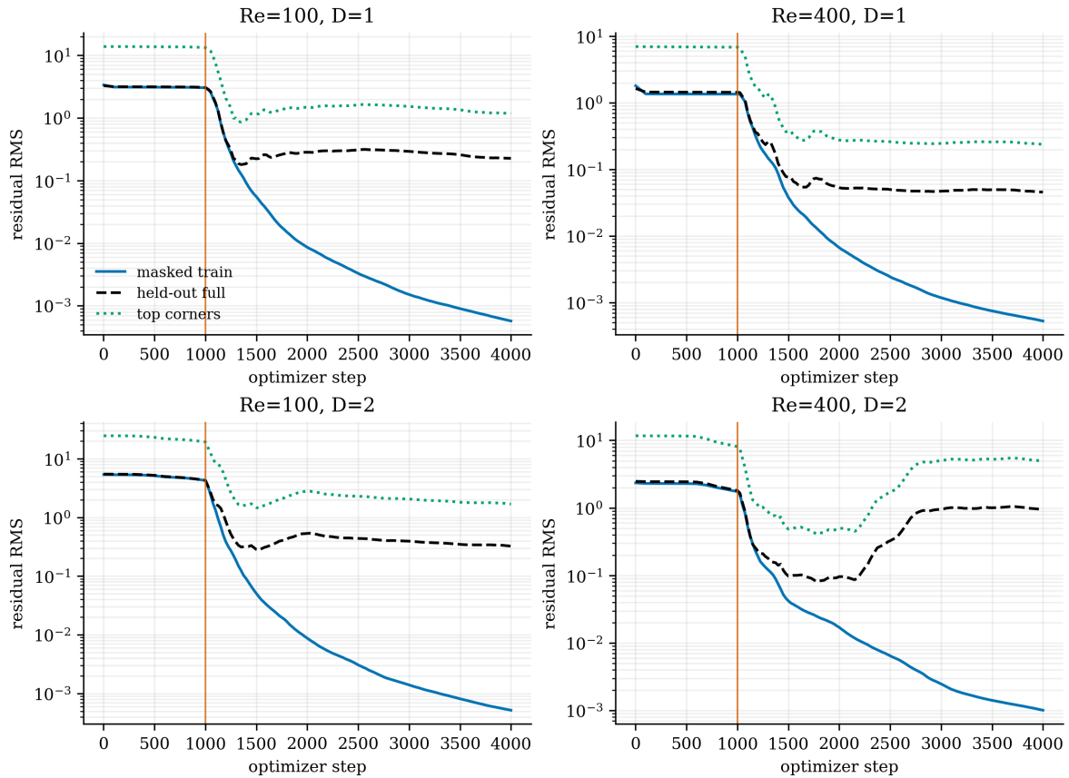
Figure 3. Adam (left of the orange line) followed by SSBroyden2. Held-out full-domain and top-corner residuals prevent masked training loss from being mistaken for global accuracy.
