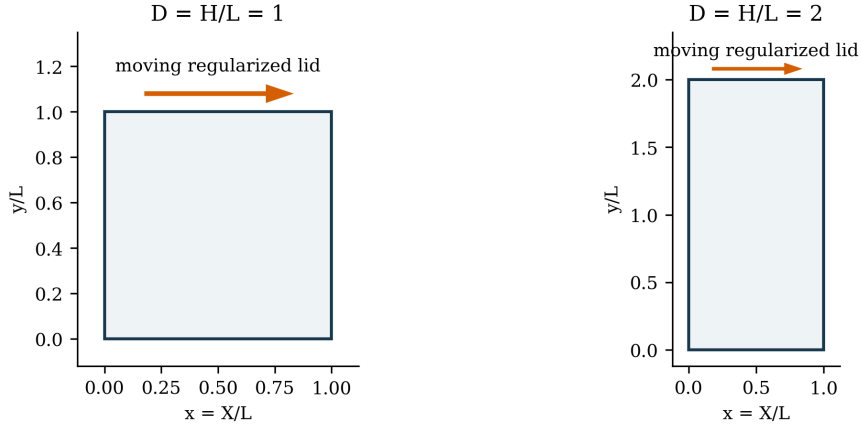
Figure 1. Width-based nondimensionalization for the square and deep cavities. The network coordinates are (x, \eta) , while physical y/L = D \eta . Equal data scales preserve geometry.
