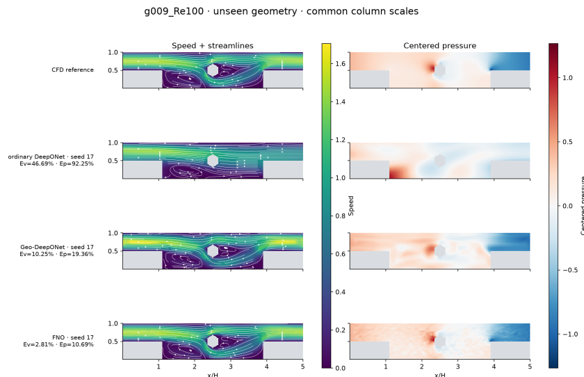
Figure 4. Unseen geometry g009 at Re=100: CFD, ordinary DeepONet, Geo-DeepONet, and FNO in rows. Row labels report seed-17 velocity and centered-pressure errors; ordinary DeepONet is markedly worse.
