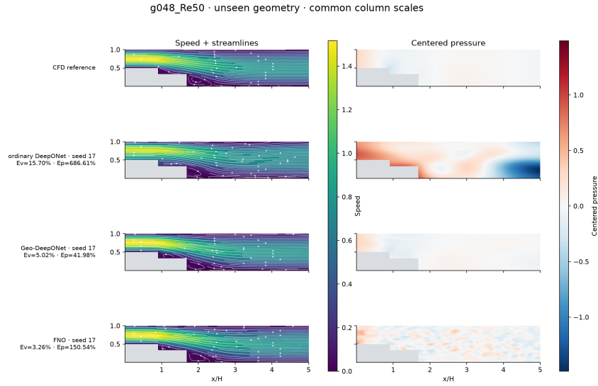
Figure 5. Unseen geometry g048 at Re=50 : the fixed-domain DeepONet is shown beside geometry-aware and spectral operators, with seed-17 errors printed in each row.
