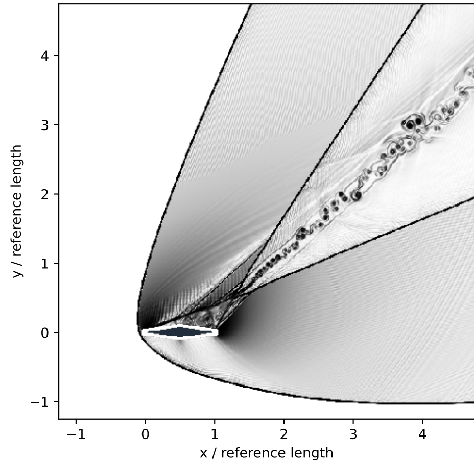
Native-density schlieren
