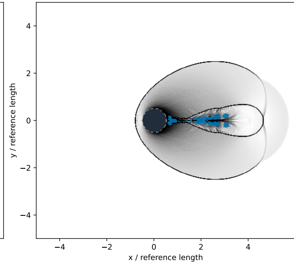
Learned vortex cores
