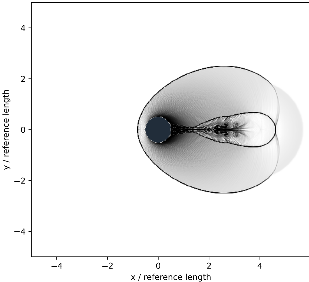
Native-density schlieren
