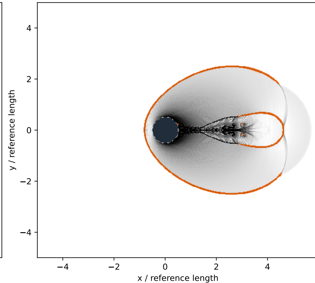
Learned shock front
