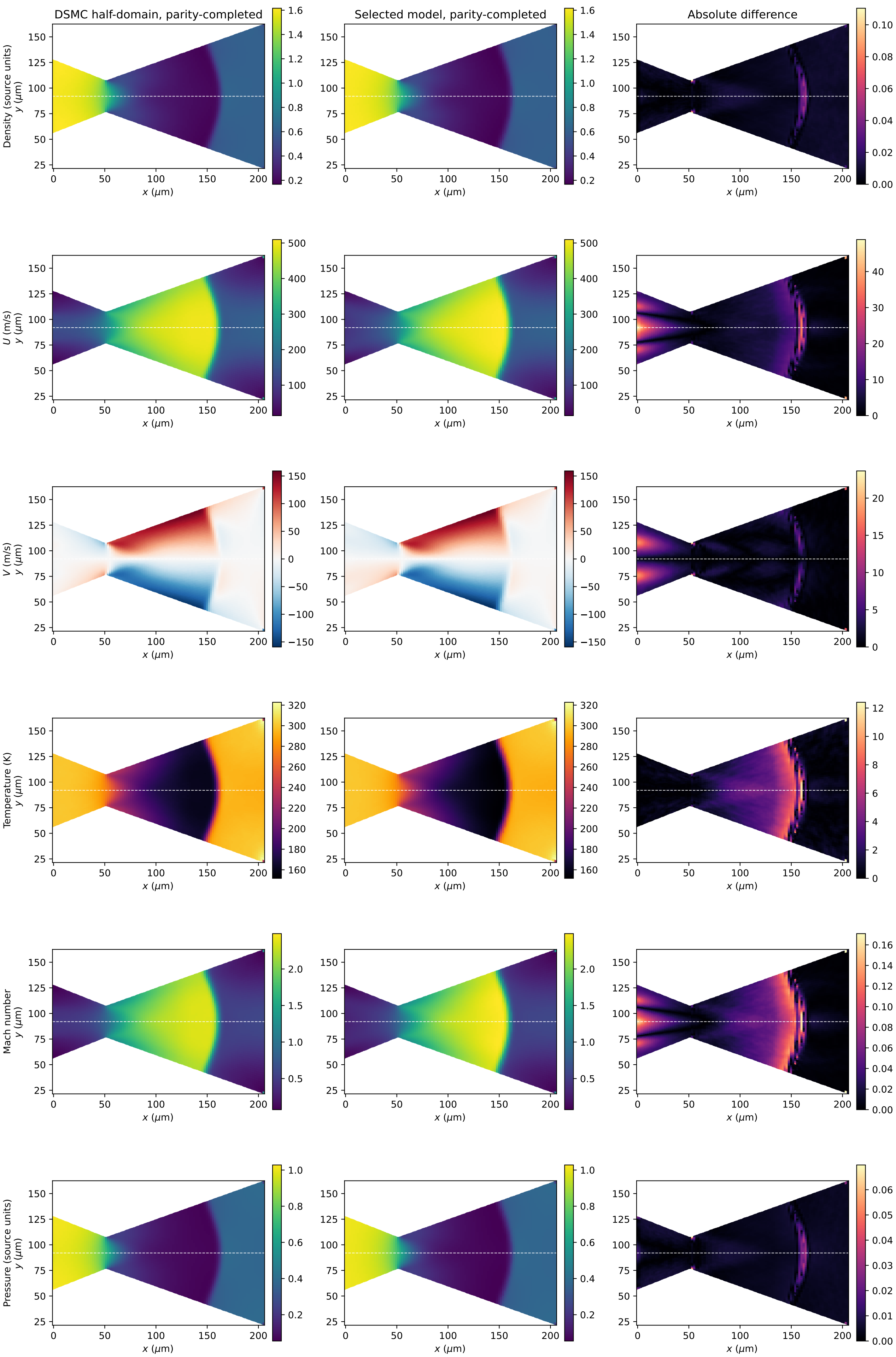
Week 9 micro-nozzle at 16 kPa | full-height parity-completed view dashed line: stated symmetry plane y = 92\text{ }\mu\text{m} ; V = 0 imposed only for this visualisation
