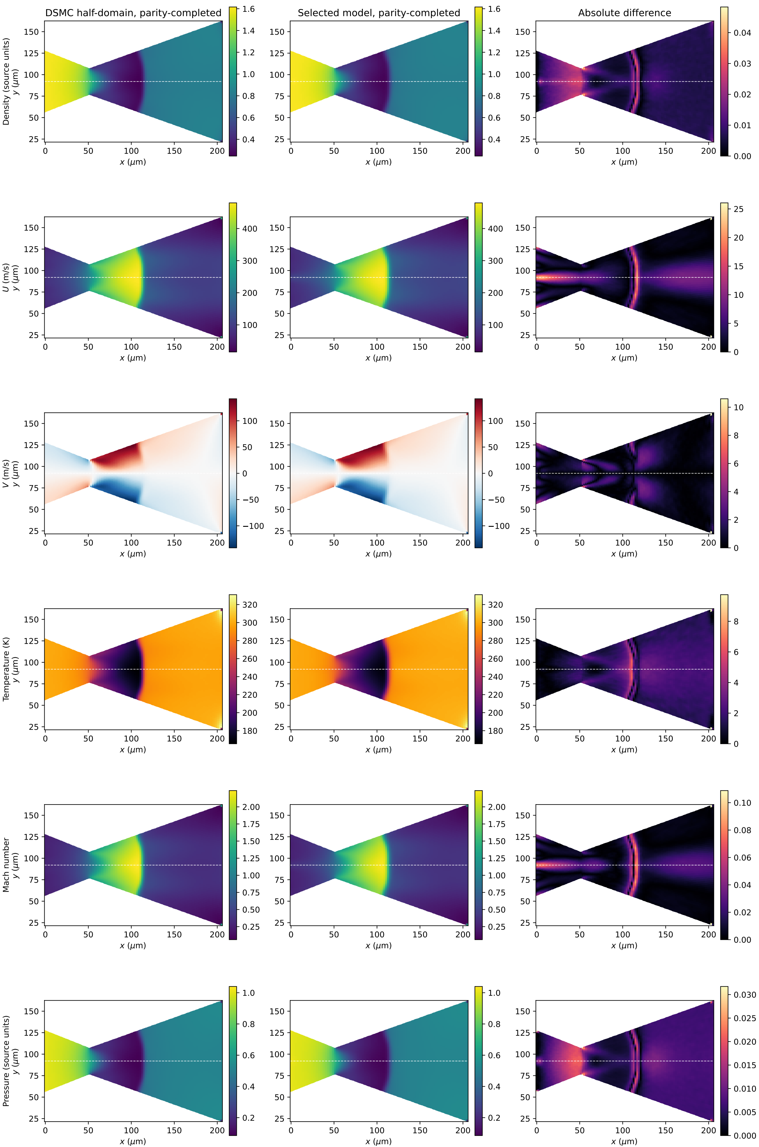
Week 9 micro-nozzle at 25 kPa | full-height parity-completed view dashed line: stated symmetry plane y = 92\text{ }\mu\text{m} ; V = 0 imposed only for this visualisation
