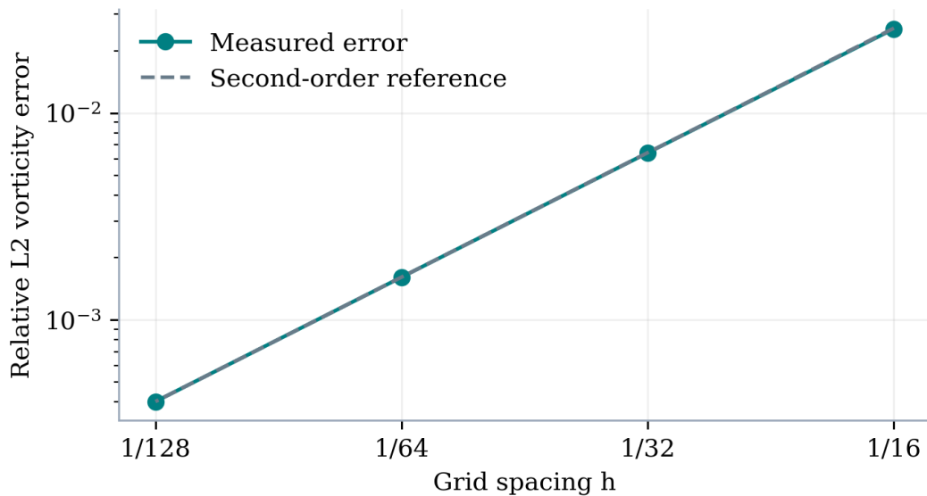
Figure 1. Error decreases at approximately second order. The reported order, 1.9965, is the slope fitted to all four log-error/log-spacing pairs.
