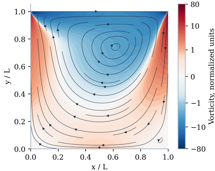
Figure 2. Vorticity computed from retained \text{Re} = 100 cavity velocities, with streamlines. Axes have equal scale. Color uses a symmetric logarithmic scale, linear within \pm 1 , to retain wall extremes while revealing the interior structure. Metrics use the support described in the text.
