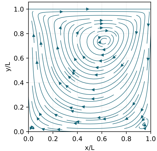
Computed streamlines
