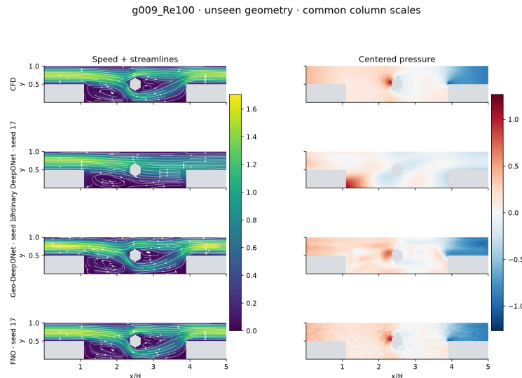
Figure 4. Unseen geometry g009 at Re=100: CFD, ordinary DeepONet, Geo-DeepONet, and FNO in rows; speed/streamlines and centered pressure in columns.
