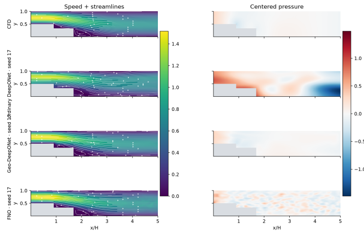
Figure 5. Unseen geometry g048 at Re=50: the fixed-domain DeepONet is shown beside geometry-aware and spectral operators.
