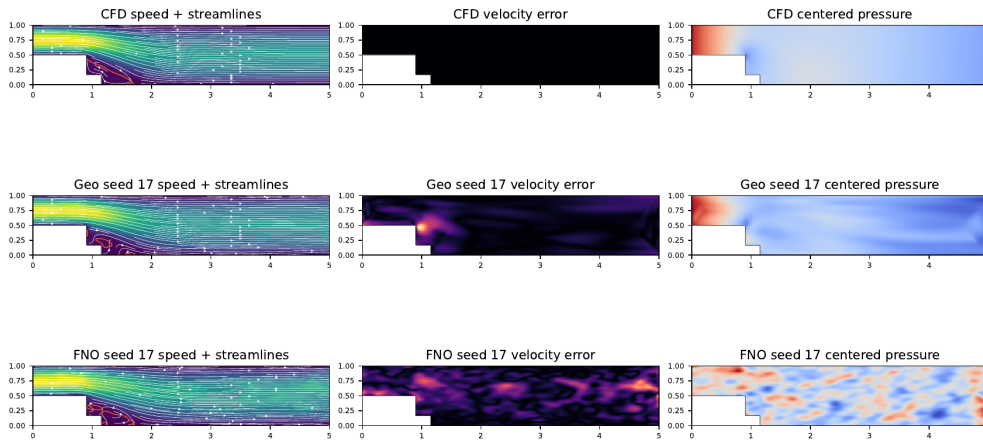
Figure 6. Whole-family holdout example g049 at Re=50 from the retained three-seed casebook.
