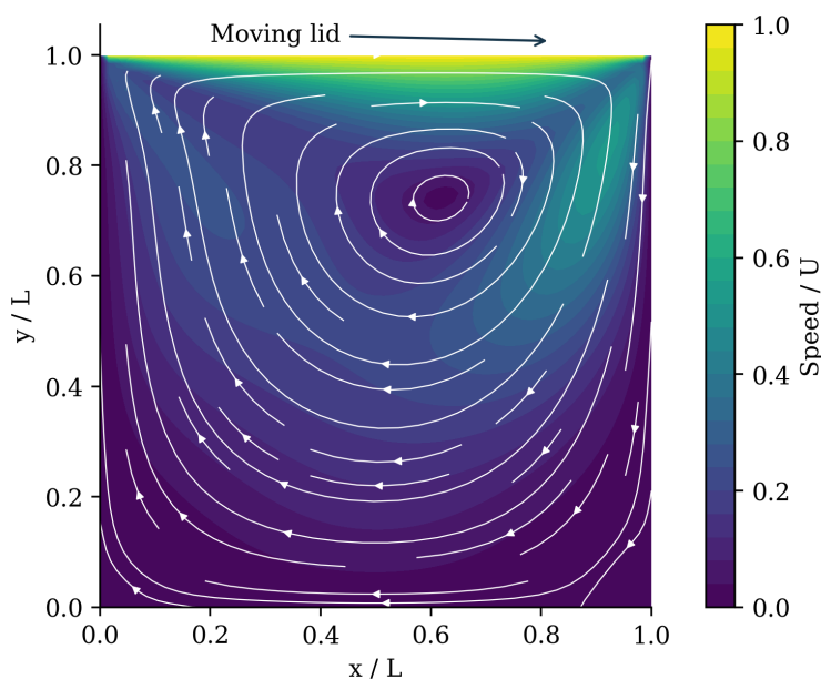
Figure 1. Retained conventional CFD field at Re=100 , with speed contours and streamlines. This is a classical-lid FlowMLLab case, not a prediction from the regularized-lid PINN. Equal axis scales preserve the square geometry.
