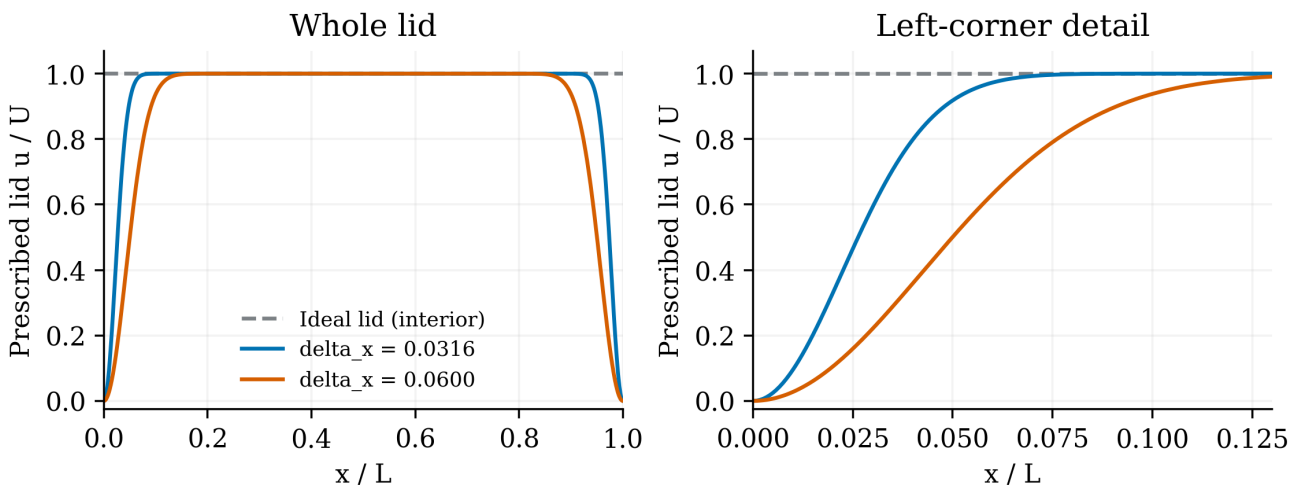
Figure 3. The analytic regularized lid profile. Blue uses the inspected upstream width; orange is an illustrative wider regularization, not another computed flow. The corner detail exposes a boundary-condition difference that a centerline plot alone could miss.
