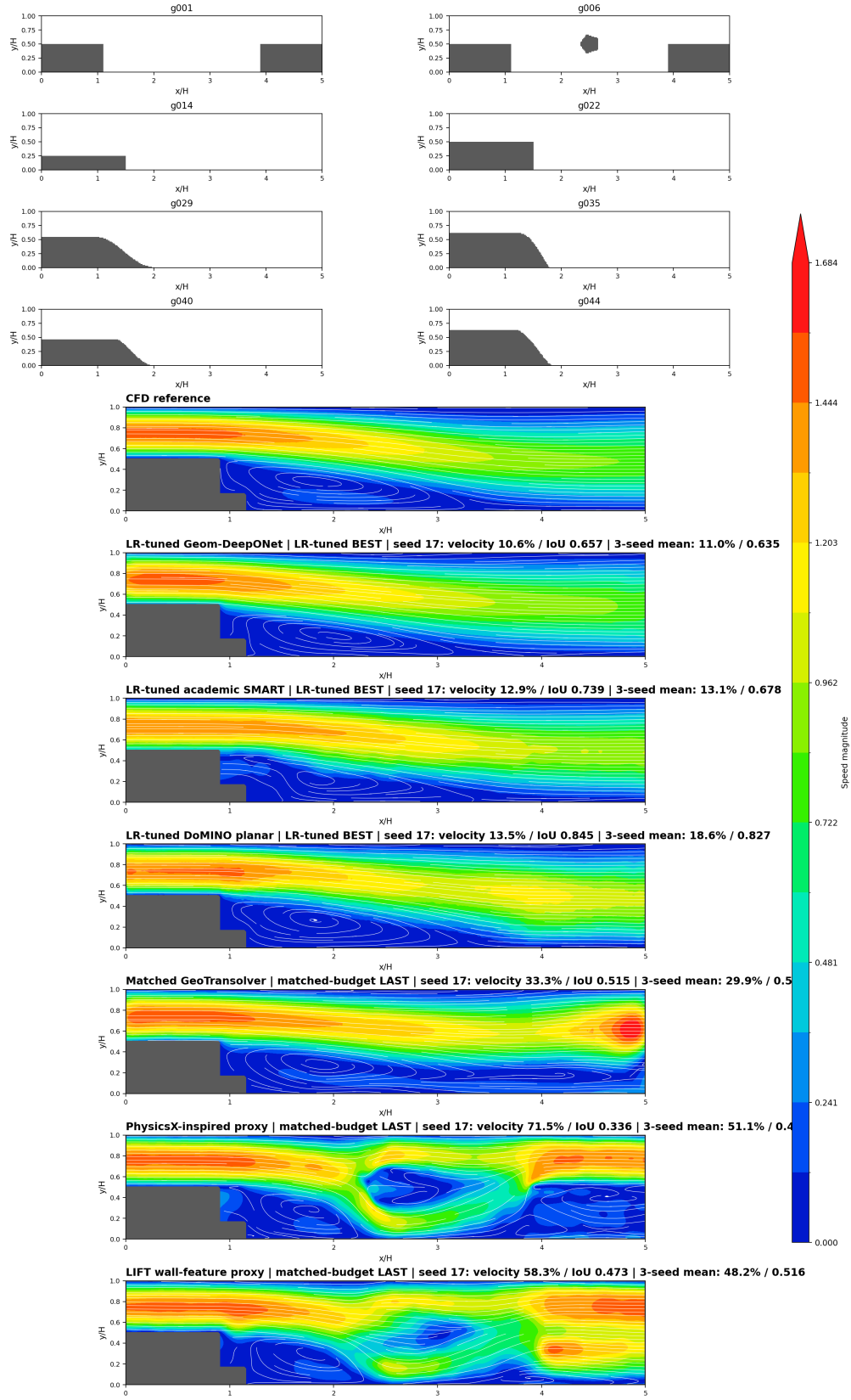
Figure 8: Extended comparison at Re=100
