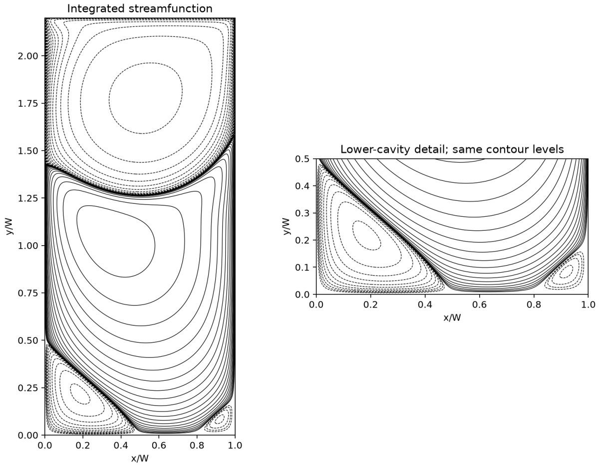
Integrated streamfunction and lower-cavity detail from checkpoint 55118. Candidate recirculation features are field diagnostics, not independently validated vortex centres.
