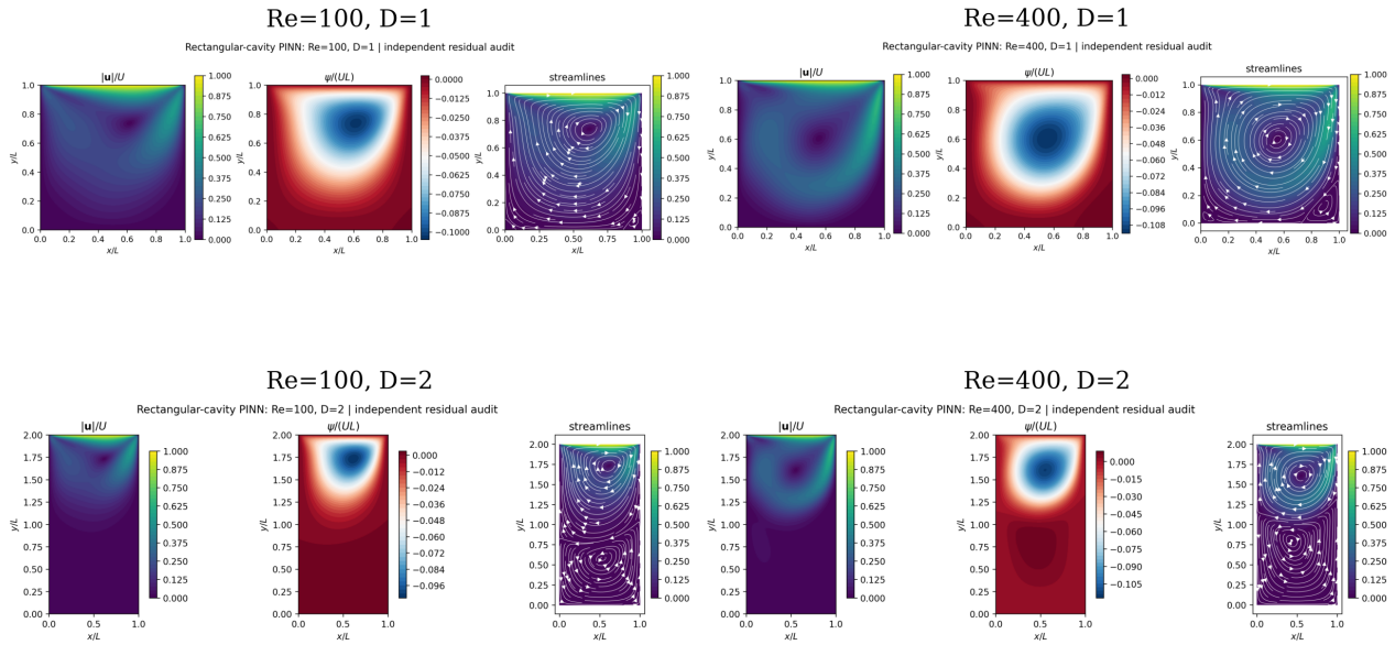
Figure 4. Retained case renders from the exact Unity jobs. These panels preserve geometric aspect ratio inside each source render. Square cases have CFD gates; deep cases are residual-audited hypotheses, not field validations.
