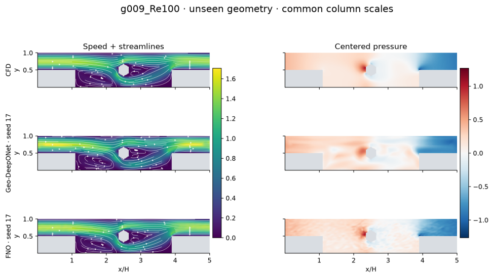
Figure 4. Unseen geometry g009 at Re=100: CFD, Geo-DeepONet, and FNO in rows; speed/streamlines and centered pressure in columns.
