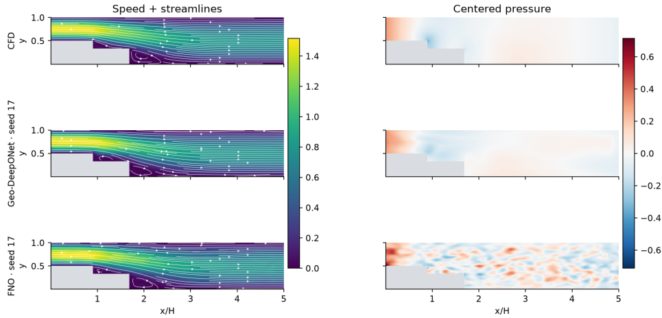
Figure 5. Unseen geometry g048 at Re=50. The FNO velocity field is competitive while pressure transfer fails.
